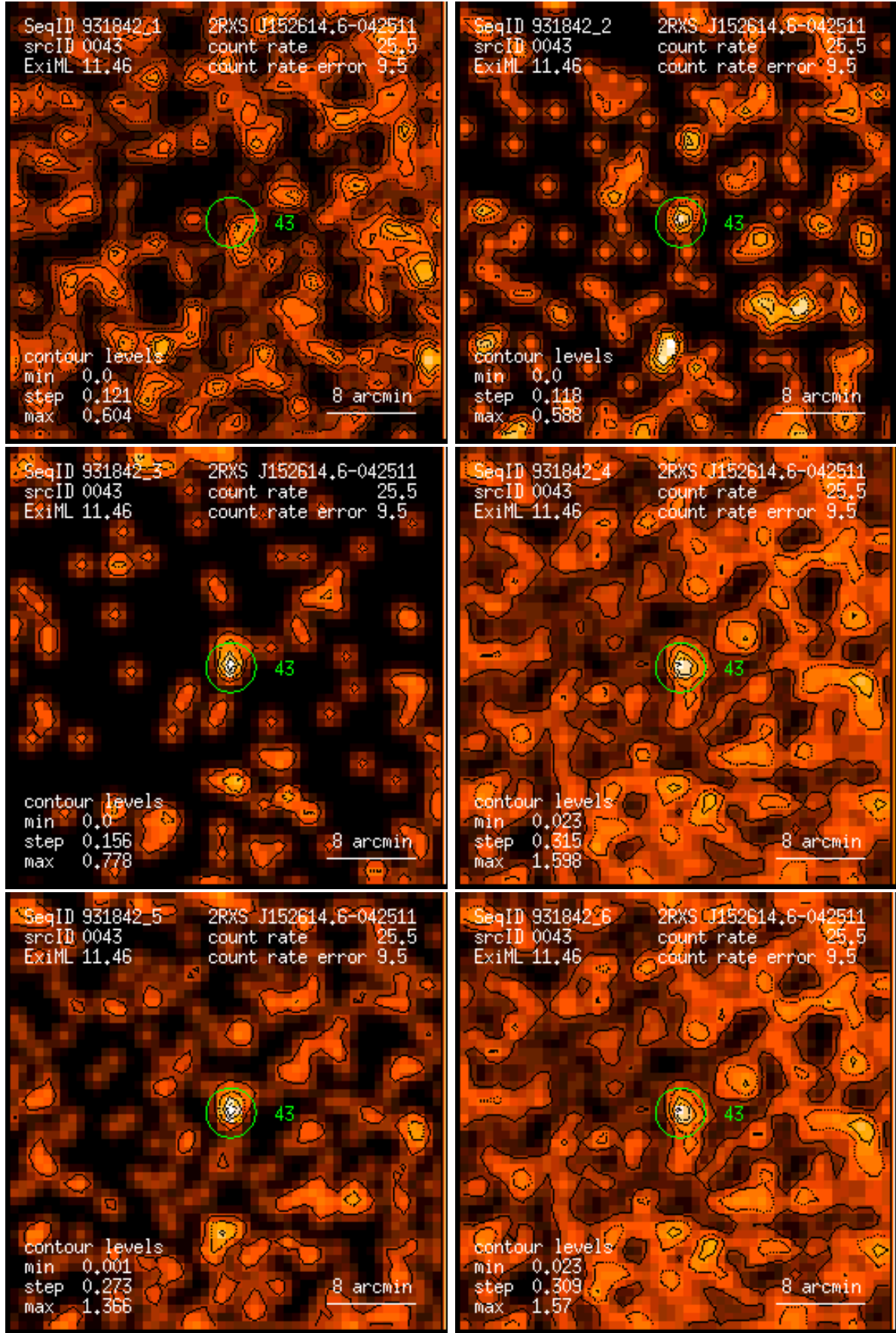
Figure 43: RASS 931842: detection 0043: band rate images, Gaussian filter: (1) PSPC channels 11 – 41, (2) 52 – 90, (3) 91 – 201, (4) 11 – 235, (5) 52 – 201, (6) 11 – 201. Broad band rates in counts/ks. Band rate contour levels in counts/ks/arcmin 2 .
