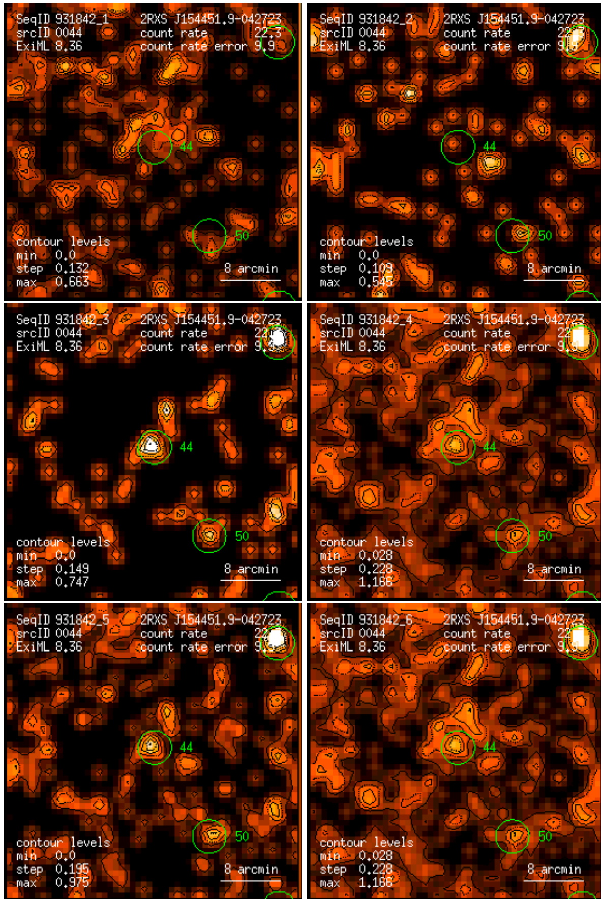
Figure 44: RASS 931842: detection 0044: band rate images, Gaussian filter: (1) PSPC channels 11 – 41, (2) 52 – 90, (3) 91 – 201, (4) 11 – 235, (5) 52 – 201, (6) 11 – 201. Broad band rates in counts/ks. Band rate contour levels in counts/ks/arcmin 2 .
