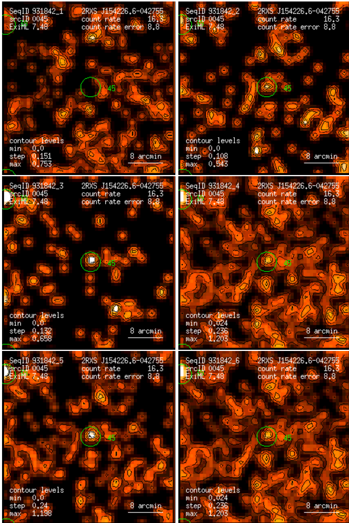
Figure 45: RASS 931842: detection 0045: band rate images, Gaussian filter: (1) PSPC channels 11 – 41, (2) 52 – 90, (3) 91 – 201, (4) 11 – 235, (5) 52 – 201, (6) 11 – 201. Broad band rates in counts/ks. Band rate contour levels in counts/ks/arcmin 2 .
