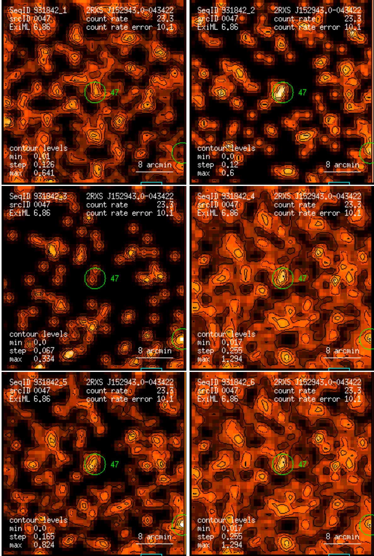
Figure 47: RASS 931842: detection 0047: band rate images, Gaussian filter: (1) PSPC channels 11 – 41, (2) 52 – 90, (3) 91 – 201, (4) 11 – 235, (5) 52 – 201, (6) 11 – 201. Broad band rates in counts/ks. Band rate contour levels in counts/ks/arcmin 2 .
