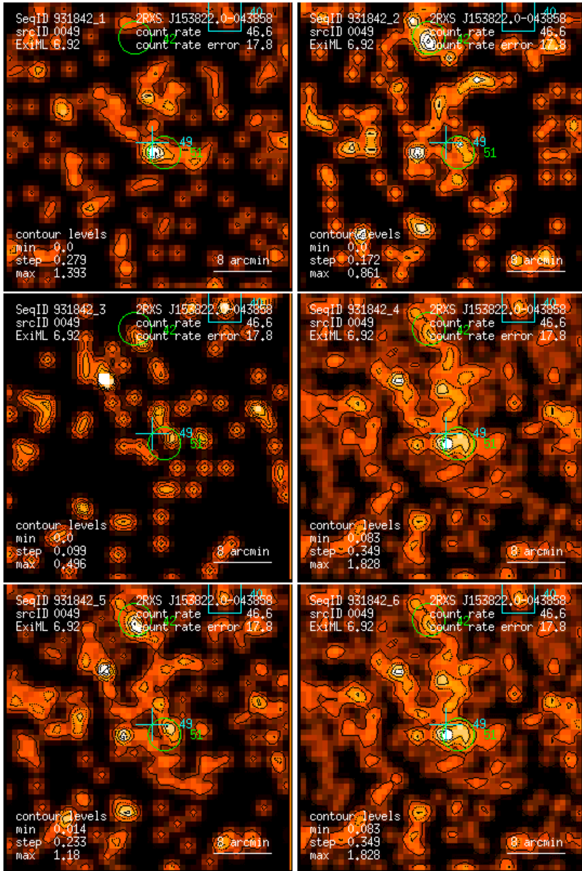
Figure 49: RASS 931842: detection 0049: band rate images, Gaussian filter: (1) PSPC channels 11 – 41, (2) 52 – 90, (3) 91 – 201, (4) 11 – 235, (5) 52 – 201, (6) 11 – 201. Broad band rates in counts/ks. Band rate contour levels in counts/ks/arcmin 2 .
