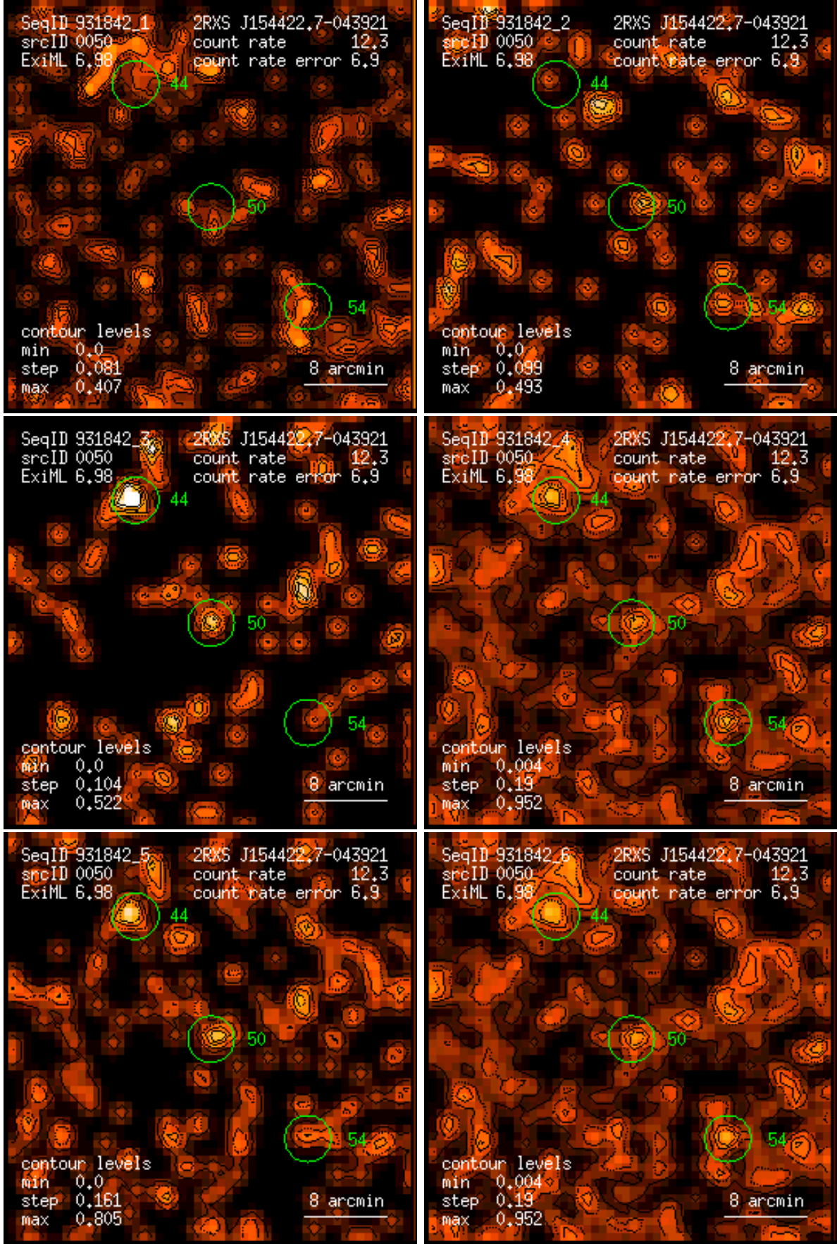
Figure 50: RASS 931842: detection 0050: band rate images, Gaussian filter: (1) PSPC channels 11 – 41, (2) 52 – 90, (3) 91 – 201, (4) 11 – 235, (5) 52 – 201, (6) 11 – 201. Broad band rates in counts/ks. Band rate contour levels in counts/ks/arcmin 2 .
