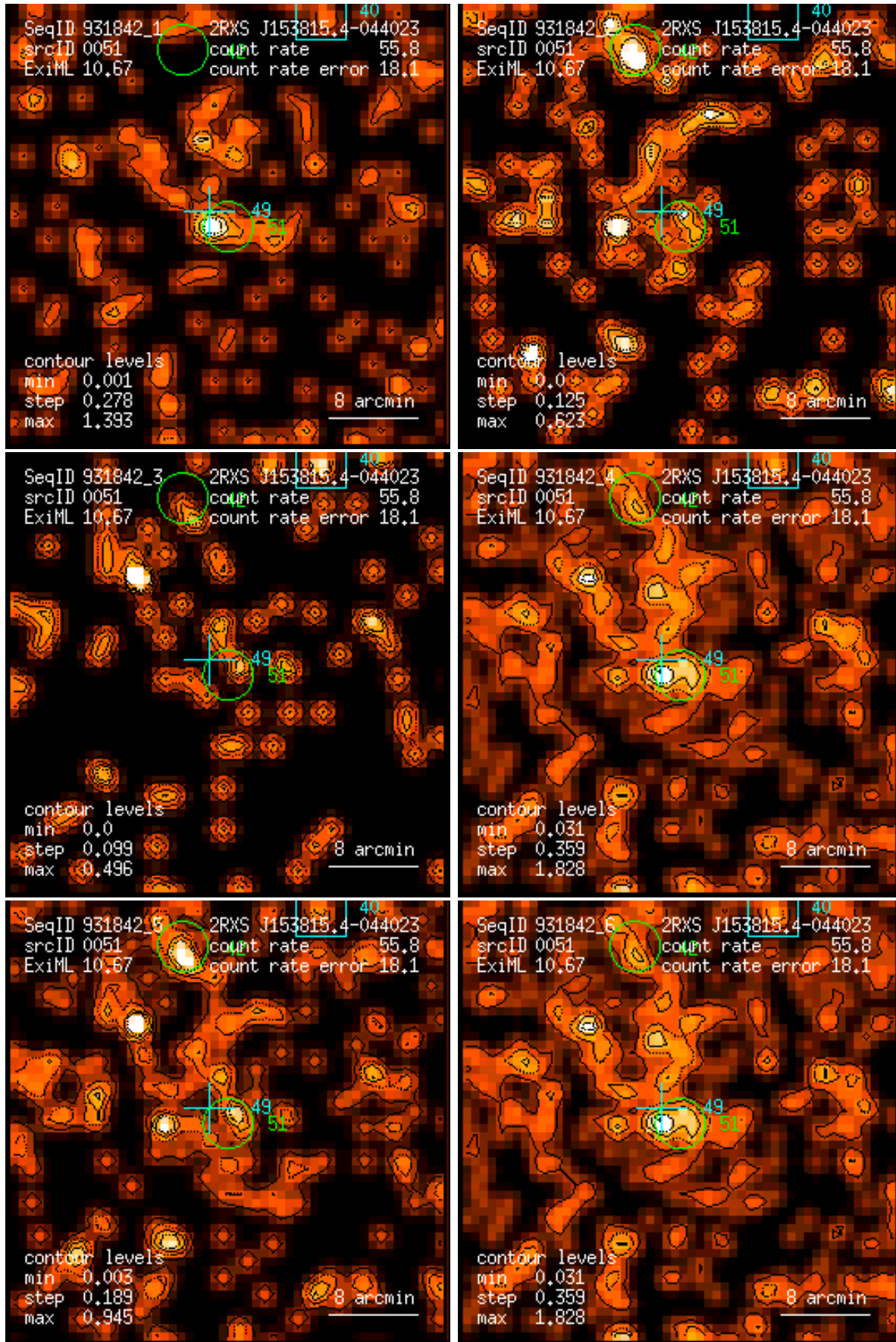
Figure 51: RASS 931842: detection 0051: band rate images, Gaussian filter: (1) PSPC channels 11 – 41, (2) 52 – 90, (3) 91 – 201, (4) 11 – 235, (5) 52 – 201, (6) 11 – 201. Broad band rates in counts/ks. Band rate contour levels in counts/ks/arcmin 2 .
