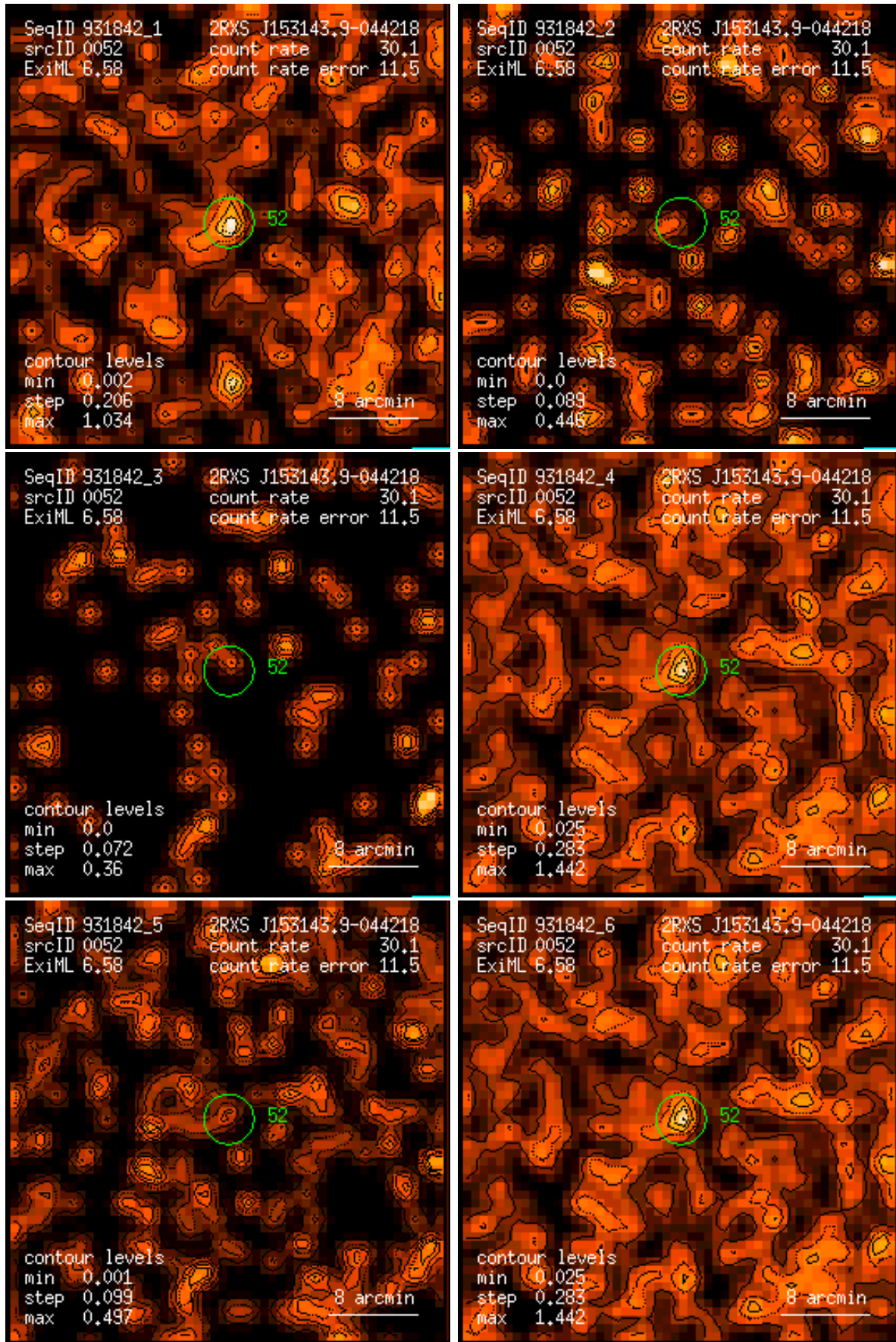
Figure 52: RASS 931842: detection 0052: band rate images, Gaussian filter: (1) PSPC channels 11 – 41, (2) 52 – 90, (3) 91 – 201, (4) 11 – 235, (5) 52 – 201, (6) 11 – 201. Broad band rates in counts/ks. Band rate contour levels in counts/ks/arcmin 2 .
