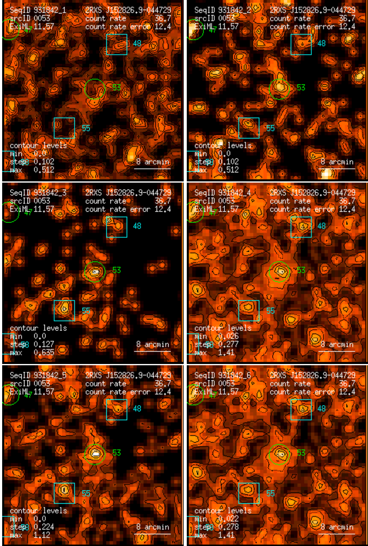
Figure 53: RASS 931842: detection 0053: band rate images, Gaussian filter: (1) PSPC channels 11 – 41, (2) 52 – 90, (3) 91 – 201, (4) 11 – 235, (5) 52 – 201, (6) 11 – 201. Broad band rates in counts/ks. Band rate contour levels in counts/ks/arcmin 2 .
