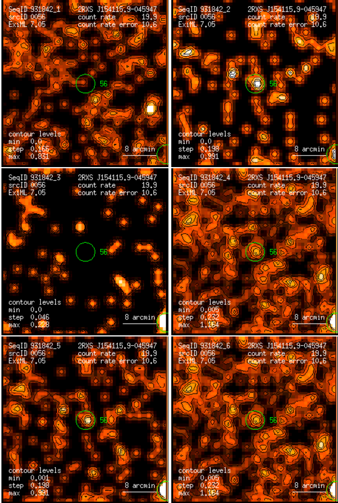
Figure 56: RASS 931842: detection 0056: band rate images, Gaussian filter: (1) PSPC channels 11 – 41, (2) 52 – 90, (3) 91 – 201, (4) 11 – 235, (5) 52 – 201, (6) 11 – 201. Broad band rates in counts/ks. Band rate contour levels in counts/ks/arcmin 2 .
