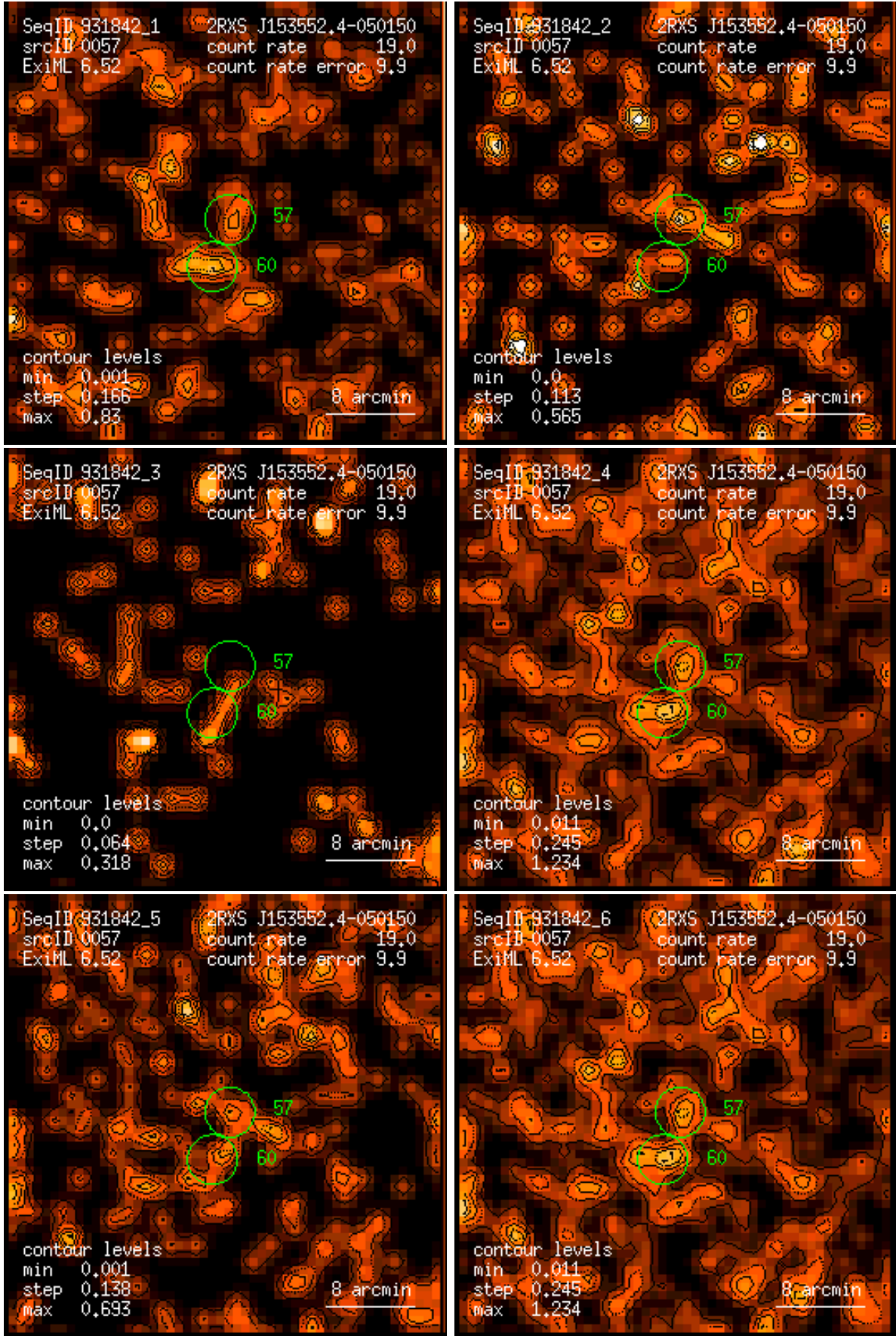
Figure 57: RASS 931842: detection 0057: band rate images, Gaussian filter: (1) PSPC channels 11 – 41, (2) 52 – 90, (3) 91 – 201, (4) 11 – 235, (5) 52 – 201, (6) 11 – 201. Broad band rates in counts/ks. Band rate contour levels in counts/ks/arcmin 2 .
