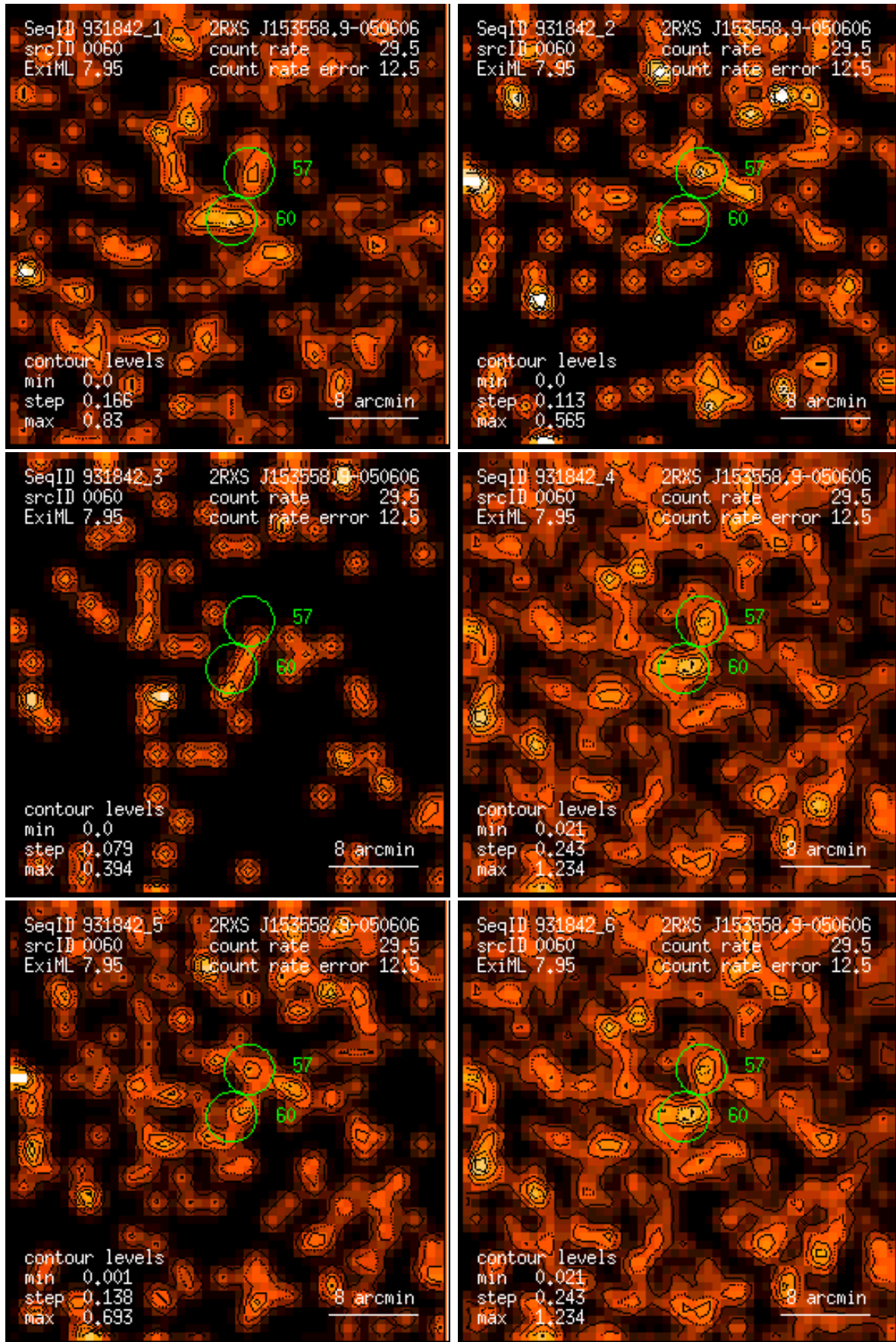
Figure 60: RASS 931842: detection 0060: band rate images, Gaussian filter: (1) PSPC channels 11 – 41, (2) 52 – 90, (3) 91 – 201, (4) 11 – 235, (5) 52 – 201, (6) 11 – 201. Broad band rates in counts/ks. Band rate contour levels in counts/ks/arcmin 2 .
