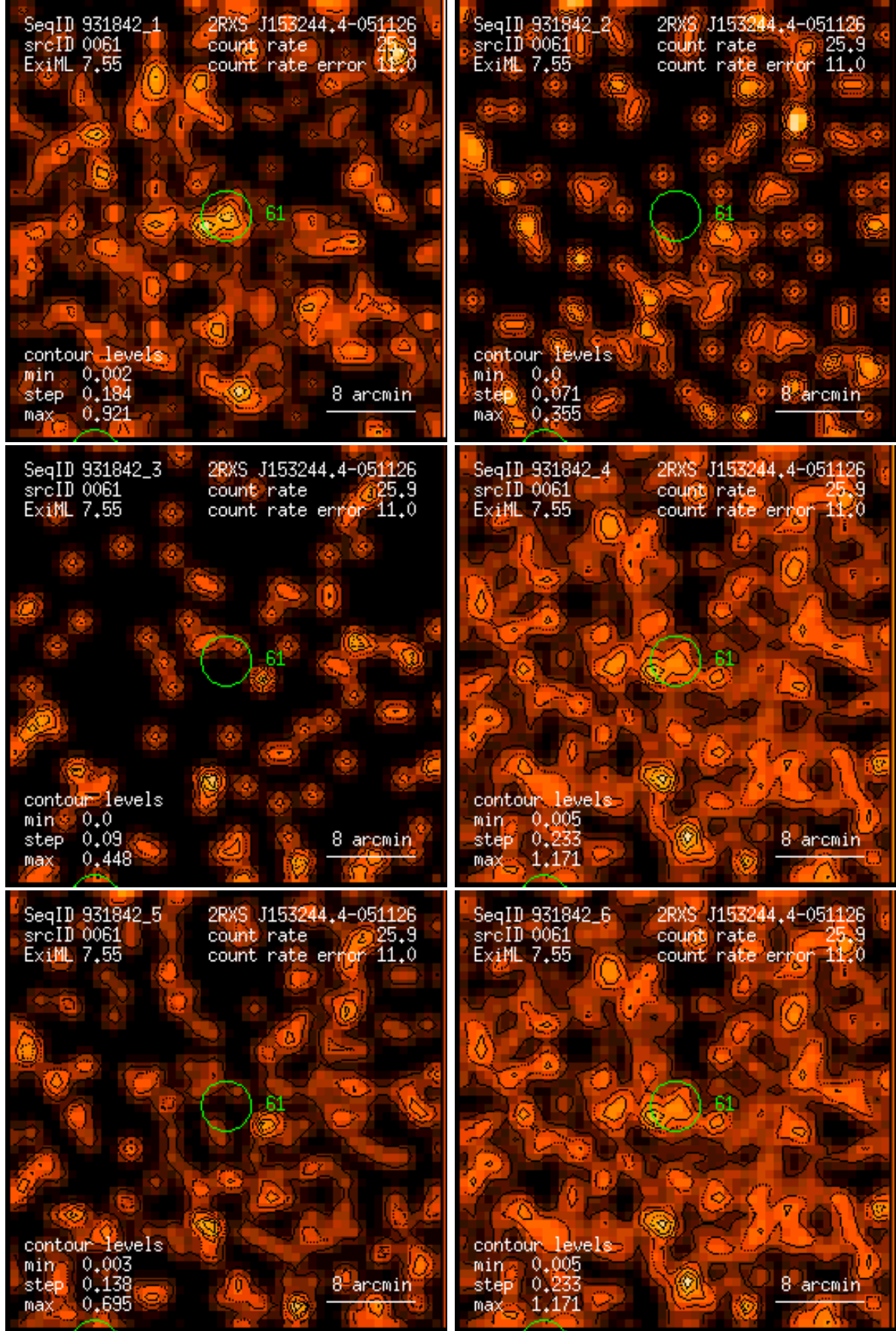
Figure 61: RASS 931842: detection 0061: band rate images, Gaussian filter: (1) PSPC channels 11 – 41, (2) 52 – 90, (3) 91 – 201, (4) 11 – 235, (5) 52 – 201, (6) 11 – 201. Broad band rates in counts/ks. Band rate contour levels in counts/ks/arcmin 2 .
