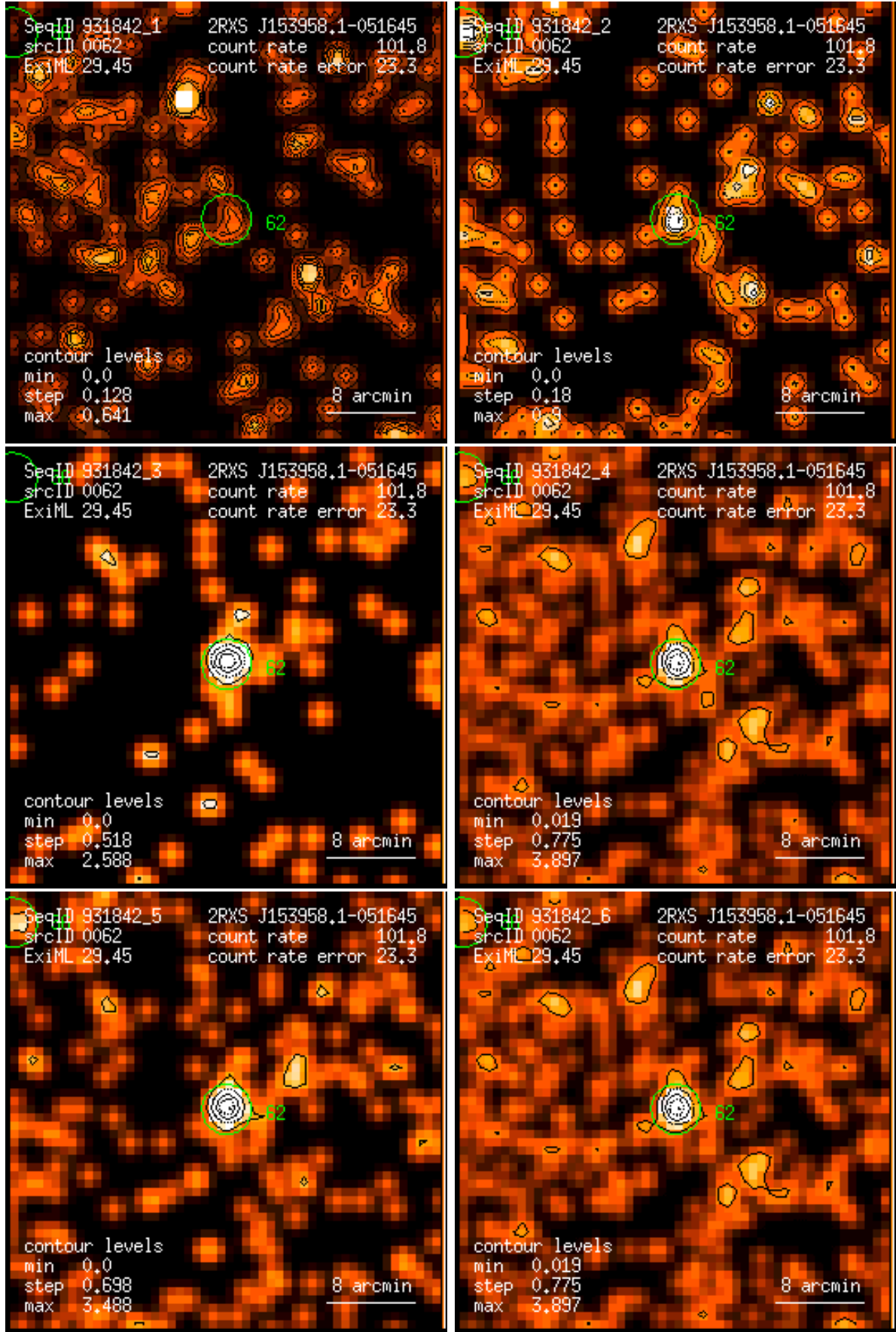
Figure 62: RASS 931842: detection 0062: band rate images, Gaussian filter: (1) PSPC channels 11 – 41, (2) 52 – 90, (3) 91 – 201, (4) 11 – 235, (5) 52 – 201, (6) 11 – 201. Broad band rates in counts/ks. Band rate contour levels in counts/ks/arcmin 2 .
