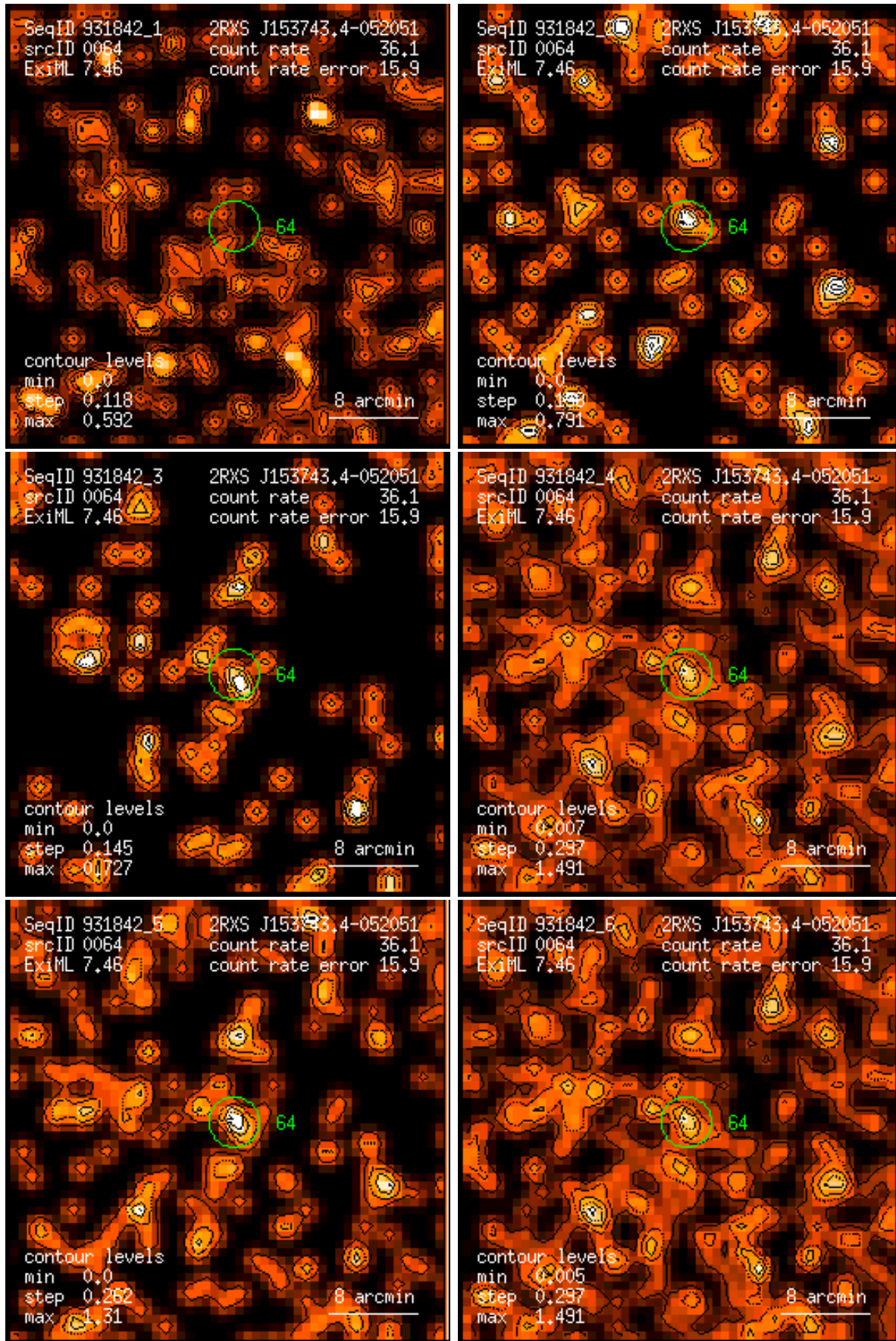
Figure 64: RASS 931842: detection 0064: band rate images, Gaussian filter: (1) PSPC channels 11 – 41, (2) 52 – 90, (3) 91 – 201, (4) 11 – 235, (5) 52 – 201, (6) 11 – 201. Broad band rates in counts/ks. Band rate contour levels in counts/ks/arcmin 2 .
