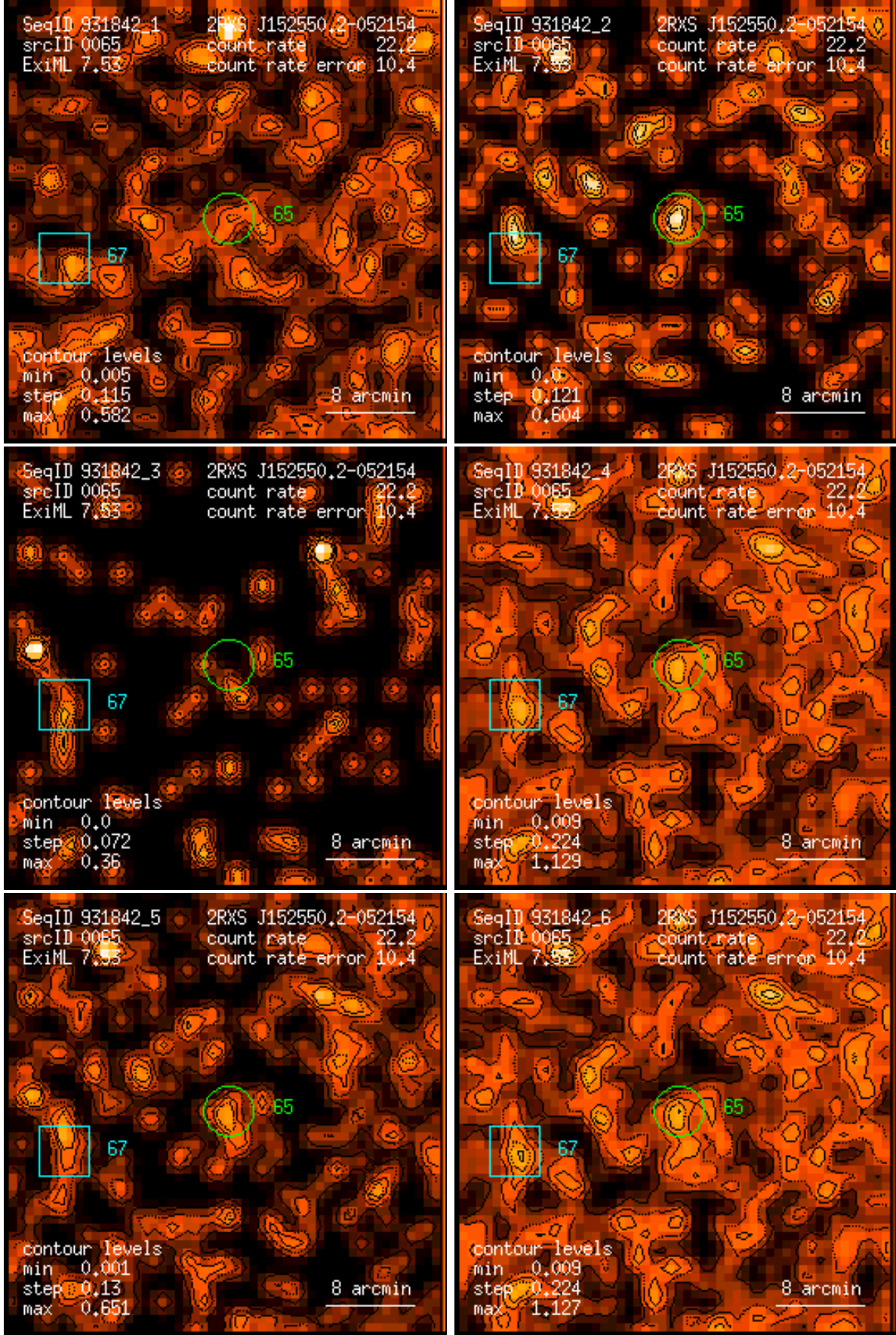
Figure 65: RASS 931842: detection 0065: band rate images, Gaussian filter: (1) PSPC channels 11 – 41, (2) 52 – 90, (3) 91 – 201, (4) 11 – 235, (5) 52 – 201, (6) 11 – 201. Broad band rates in counts/ks. Band rate contour levels in counts/ks/arcmin 2 .
