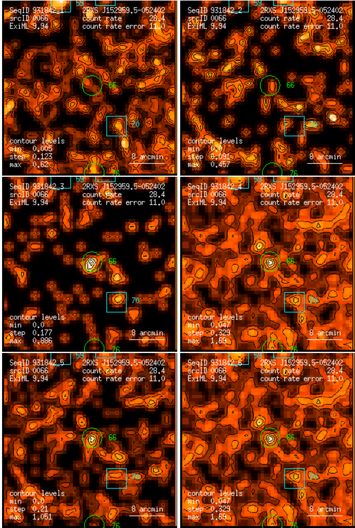
Figure 66: RASS 931842: detection 0066: band rate images, Gaussian filter: (1) PSPC channels 11 – 41, (2) 52 – 90, (3) 91 – 201, (4) 11 – 235, (5) 52 – 201, (6) 11 – 201. Broad band rates in counts/ks. Band rate contour levels in counts/ks/arcmin 2 .
