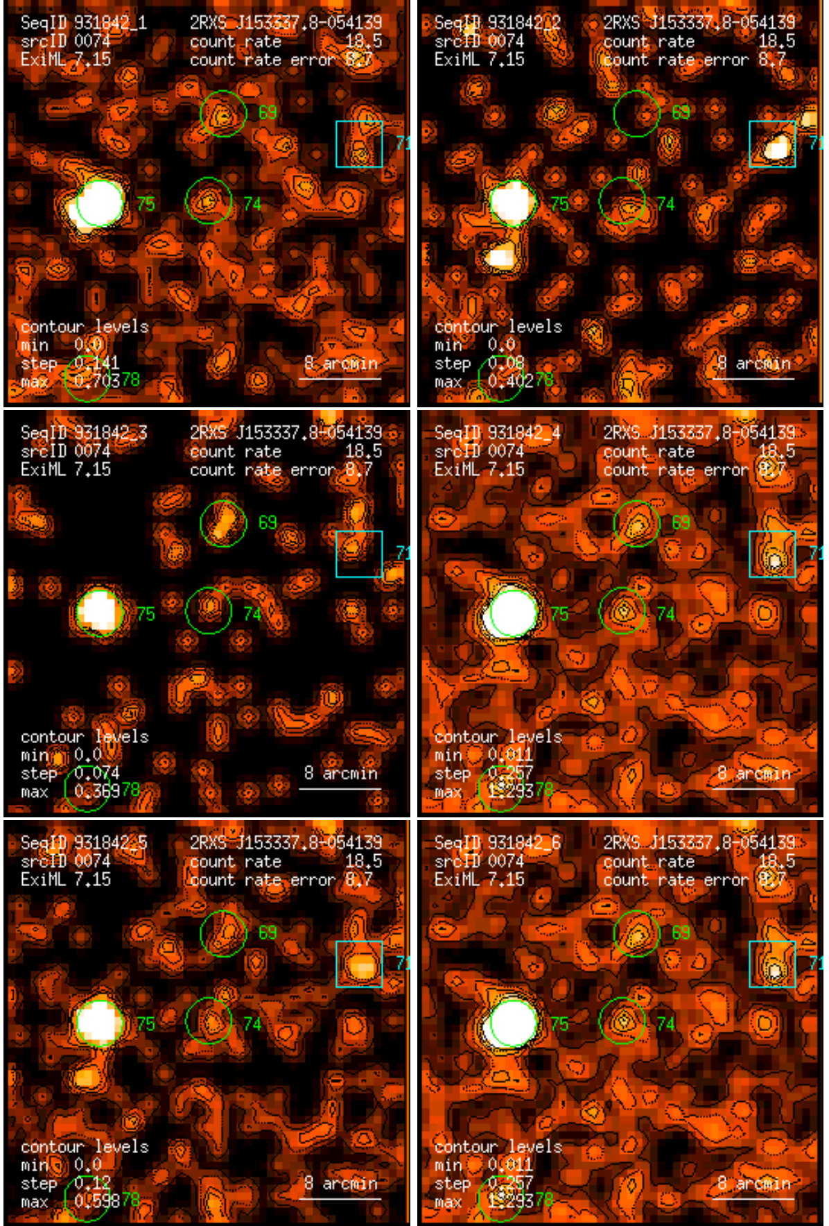
Figure 74: RASS 931842: detection 0074: band rate images, Gaussian filter: (1) PSPC channels 11 – 41, (2) 52 – 90, (3) 91 – 201, (4) 11 – 235, (5) 52 – 201, (6) 11 – 201. Broad band rates in counts/ks. Band rate contour levels in counts/ks/arcmin 2 .
