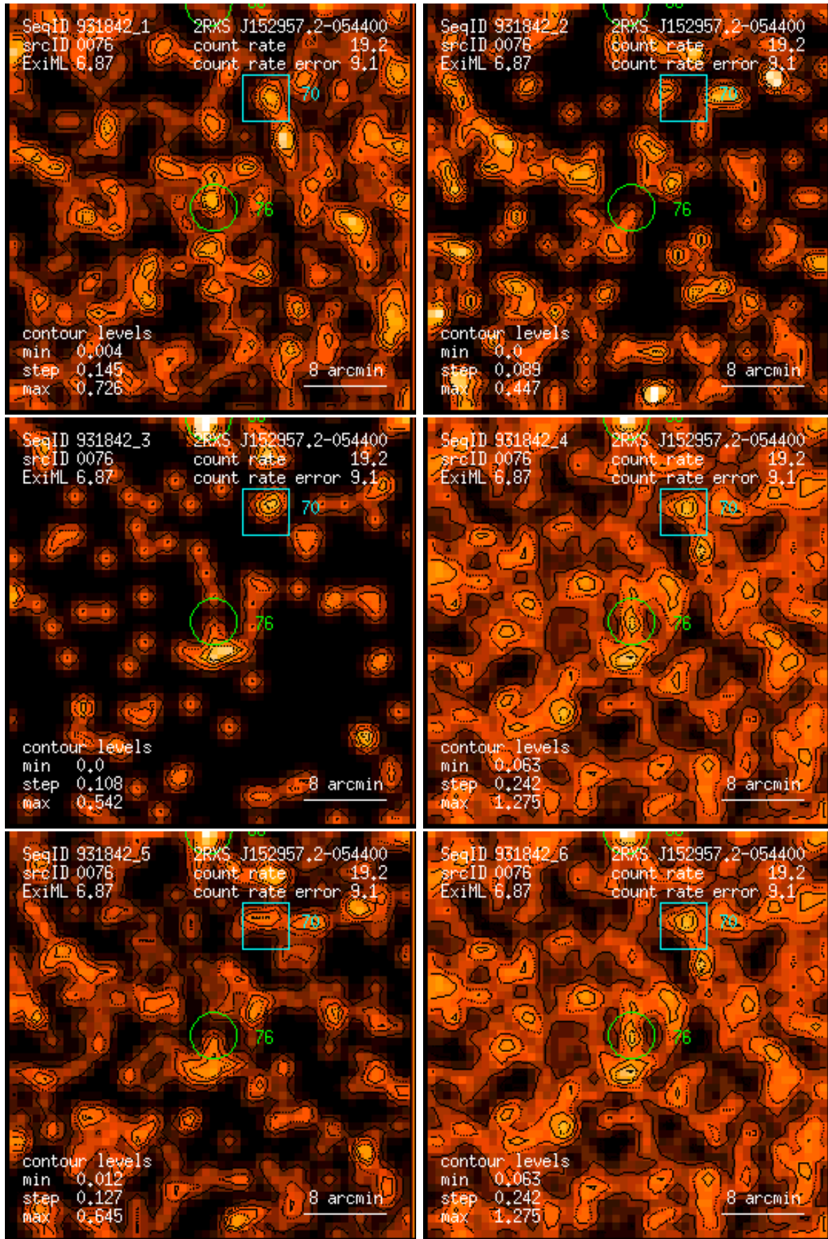
Figure 76: RASS 931842: detection 0076: band rate images, Gaussian filter: (1) PSPC channels 11 – 41, (2) 52 – 90, (3) 91 – 201, (4) 11 – 235, (5) 52 – 201, (6) 11 – 201. Broad band rates in counts/ks. Band rate contour levels in counts/ks/arcmin 2 .
