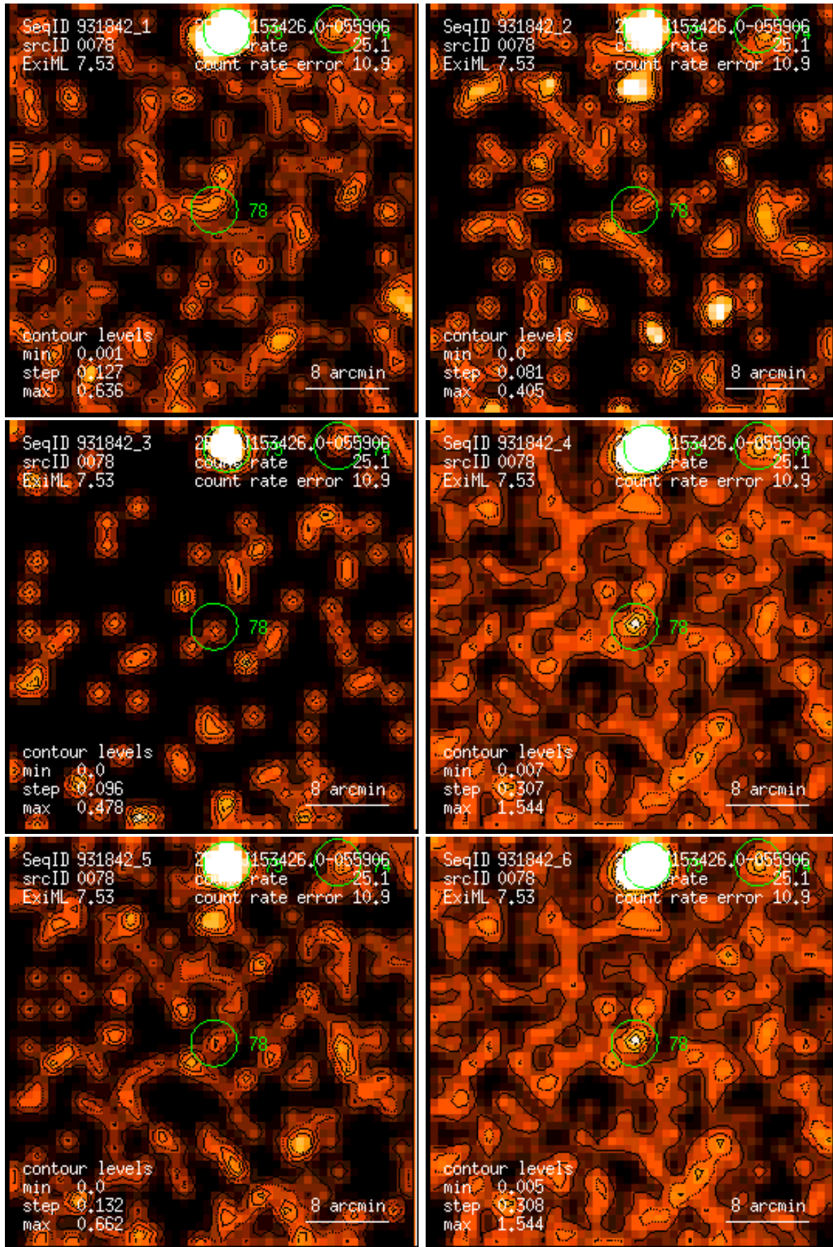
Figure 78: RASS 931842: detection 0078: band rate images, Gaussian filter: (1) PSPC channels 11 – 41, (2) 52 – 90, (3) 91 – 201, (4) 11 – 235, (5) 52 – 201, (6) 11 – 201. Broad band rates in counts/ks. Band rate contour levels in counts/ks/arcmin 2 .
