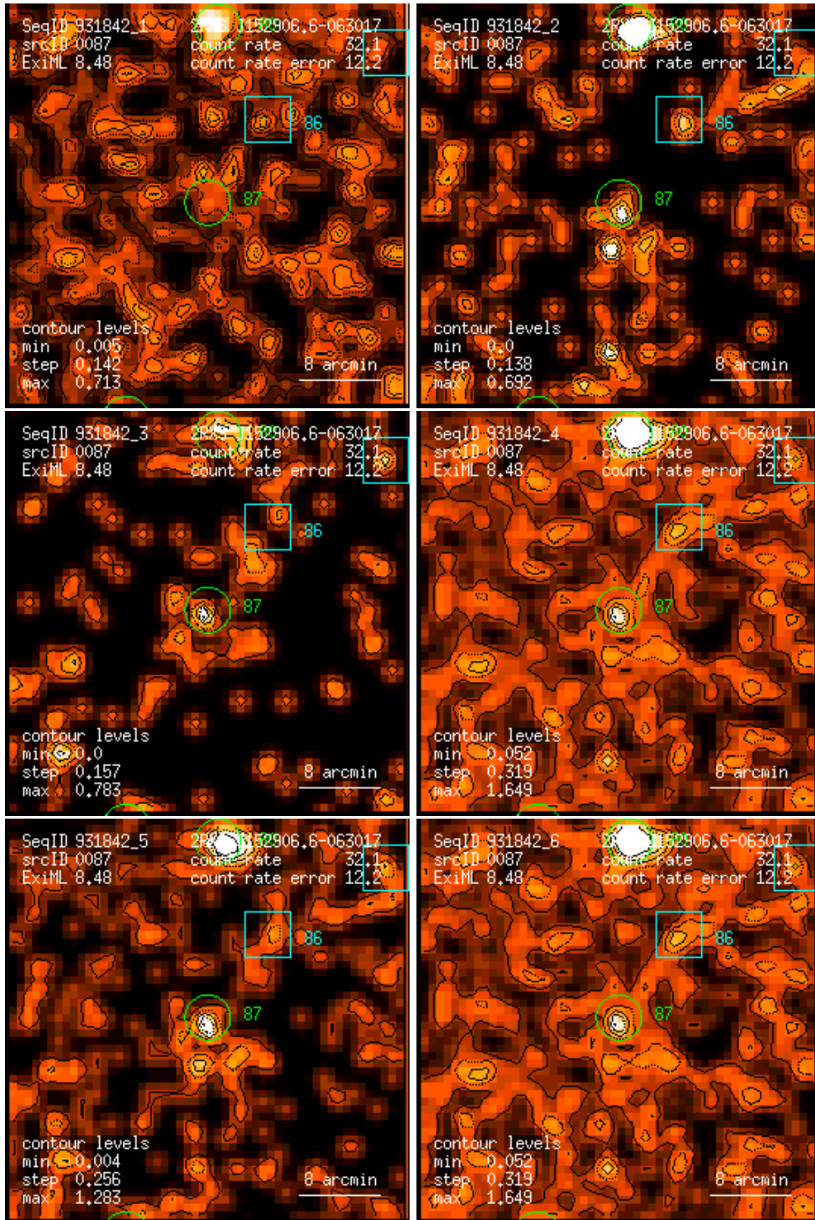
Figure 87: RASS 931842: detection 0087: band rate images, Gaussian filter: (1) PSPC channels 11 – 41, (2) 52 – 90, (3) 91 – 201, (4) 11 – 235, (5) 52 – 201, (6) 11 – 201. Broad band rates in counts/ks. Band rate contour levels in counts/ks/arcmin 2 .
