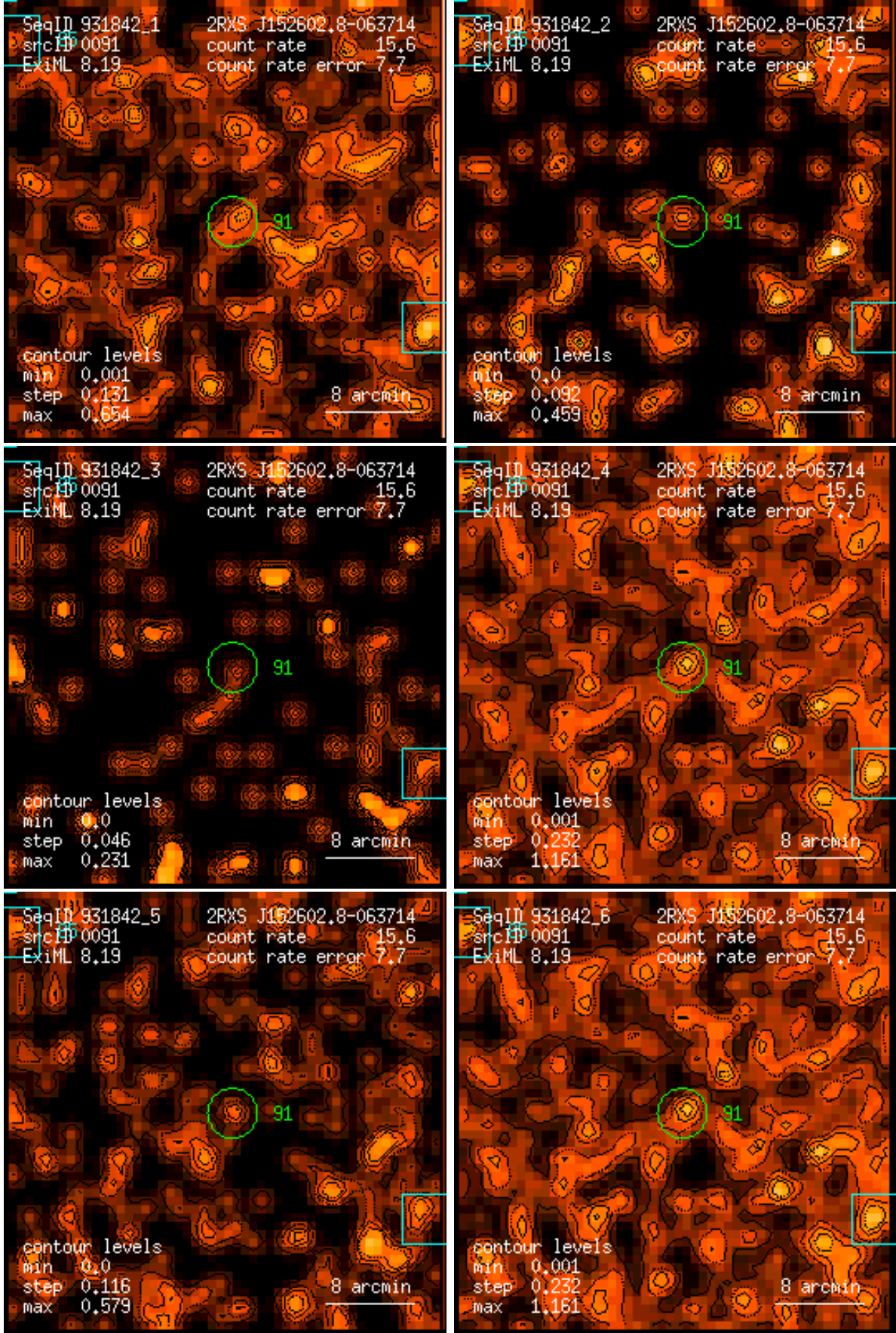
Figure 91: RASS 931842: detection 0091: band rate images, Gaussian filter: (1) PSPC channels 11 – 41, (2) 52 – 90, (3) 91 – 201, (4) 11 – 235, (5) 52 – 201, (6) 11 – 201. Broad band rates in counts/ks. Band rate contour levels in counts/ks/arcmin 2 .
