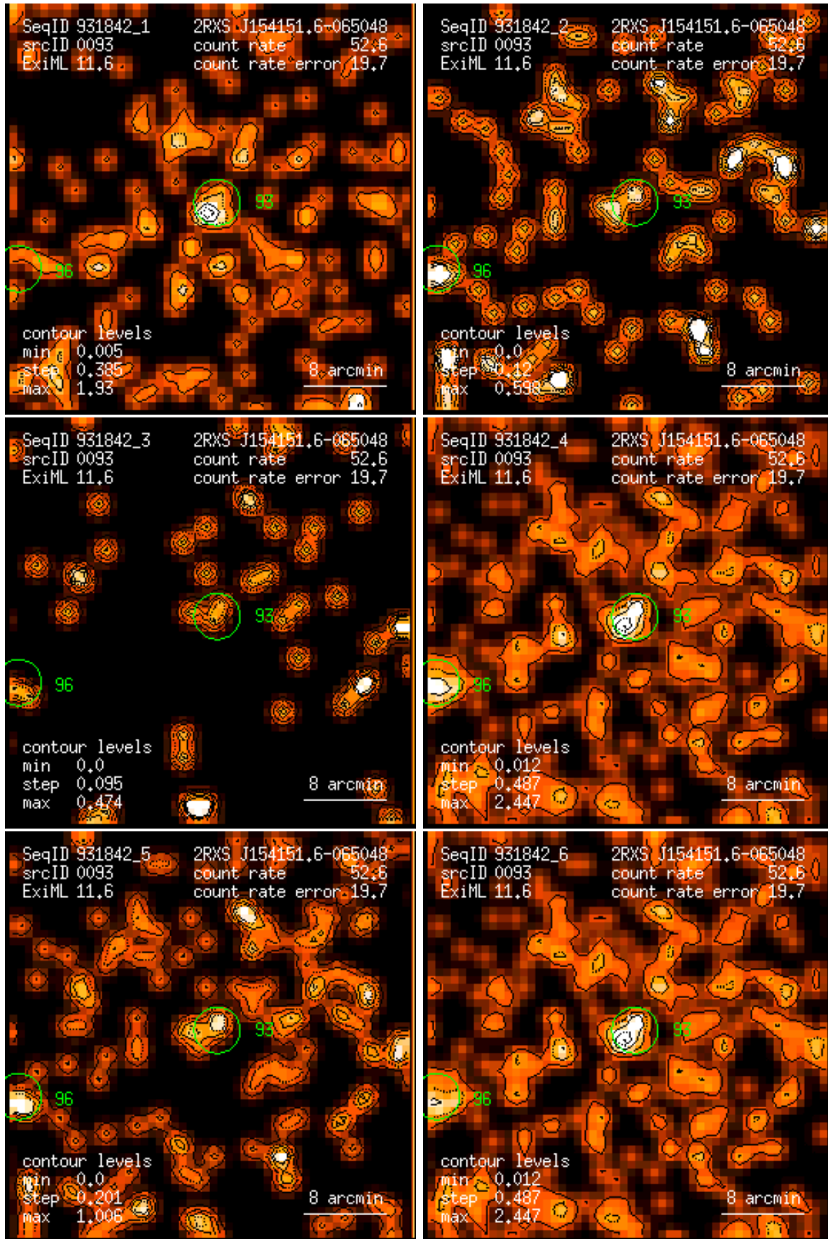
Figure 93: RASS 931842: detection 0093: band rate images, Gaussian filter: (1) PSPC channels 11 – 41, (2) 52 – 90, (3) 91 – 201, (4) 11 – 235, (5) 52 – 201, (6) 11 – 201. Broad band rates in counts/ks. Band rate contour levels in counts/ks/arcmin 2 .
