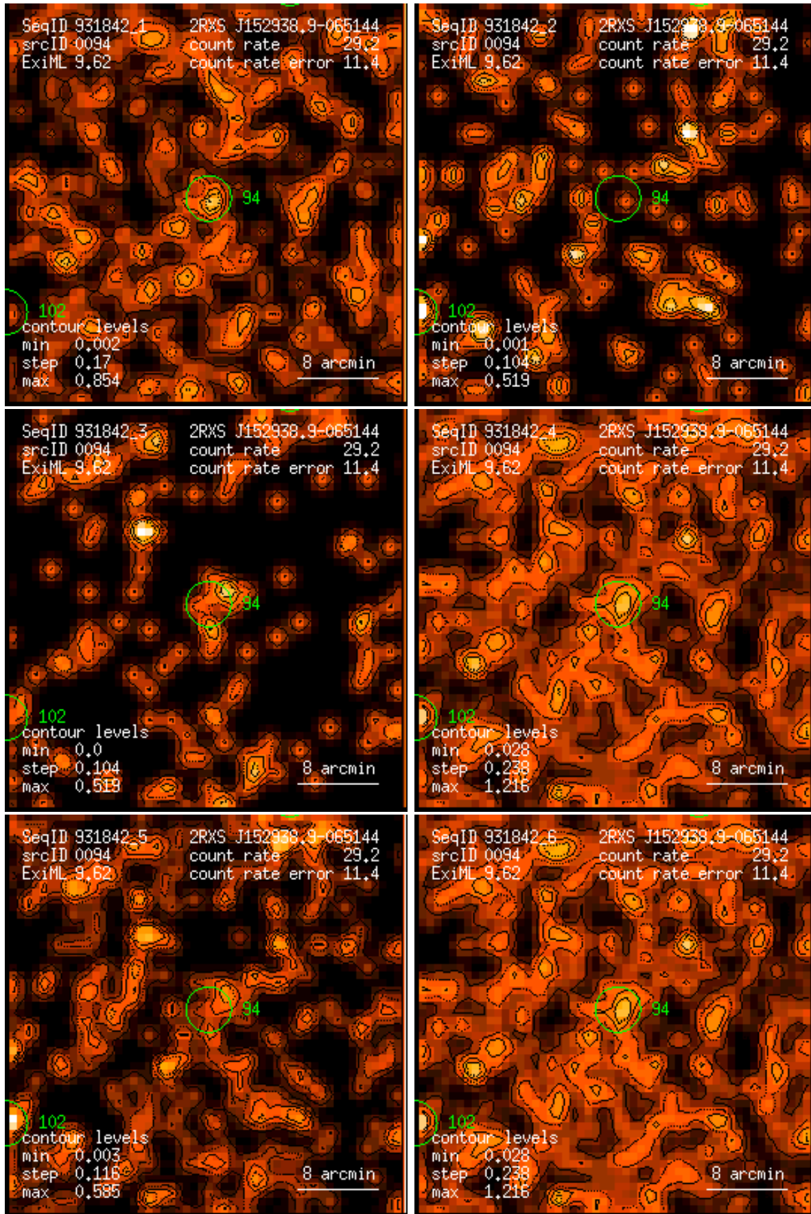
Figure 94: RASS 931842: detection 0094: band rate images, Gaussian filter: (1) PSPC channels 11 – 41, (2) 52 – 90, (3) 91 – 201, (4) 11 – 235, (5) 52 – 201, (6) 11 – 201. Broad band rates in counts/ks. Band rate contour levels in counts/ks/arcmin 2 .
