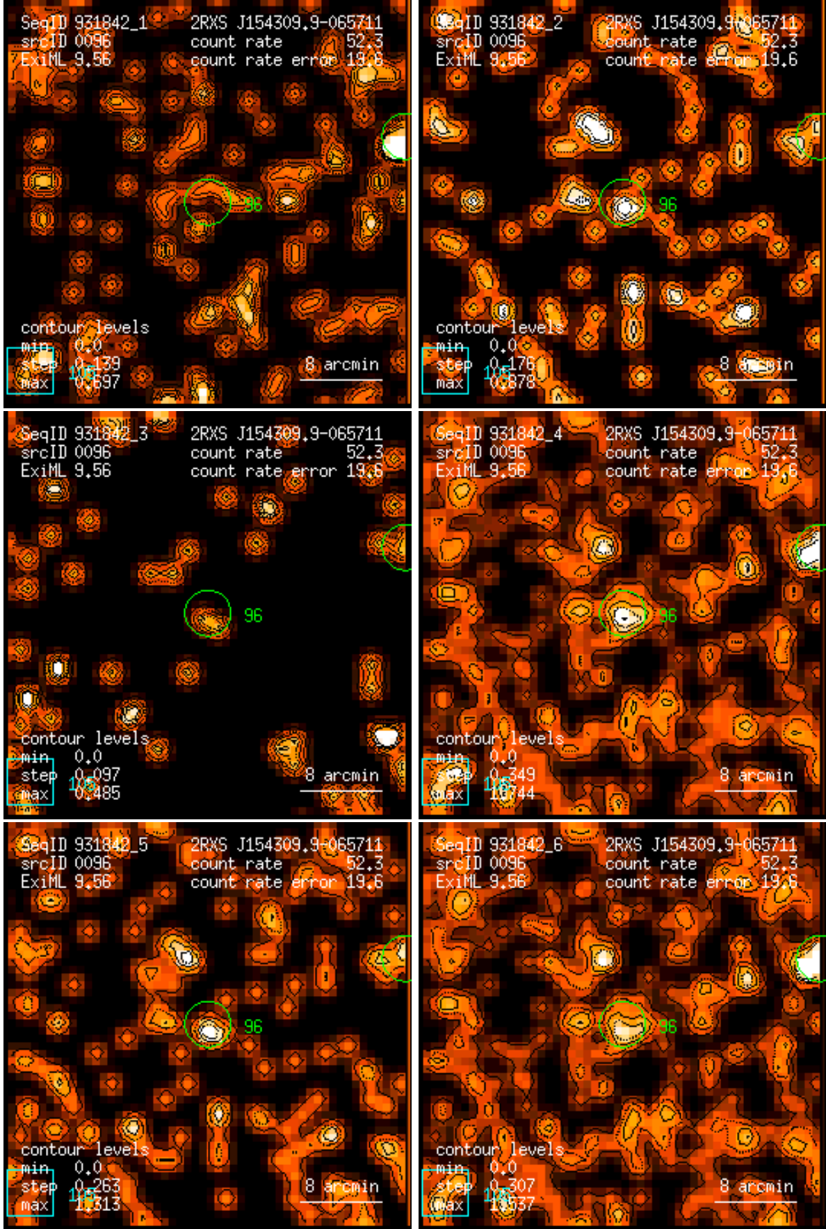
Figure 96: RASS 931842: detection 0096: band rate images, Gaussian filter: (1) PSPC channels 11 – 41, (2) 52 – 90, (3) 91 – 201, (4) 11 – 235, (5) 52 – 201, (6) 11 – 201. Broad band rates in counts/ks. Band rate contour levels in counts/ks/arcmin 2 .
