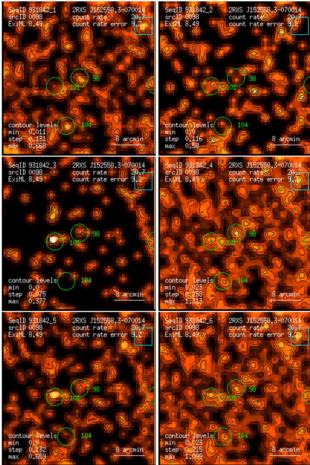
Figure 98: RASS 931842: detection 0098: band rate images, Gaussian filter: (1) PSPC channels 11 – 41, (2) 52 – 90, (3) 91 – 201, (4) 11 – 235, (5) 52 – 201, (6) 11 – 201. Broad band rates in counts/ks. Band rate contour levels in counts/ks/arcmin 2 .
