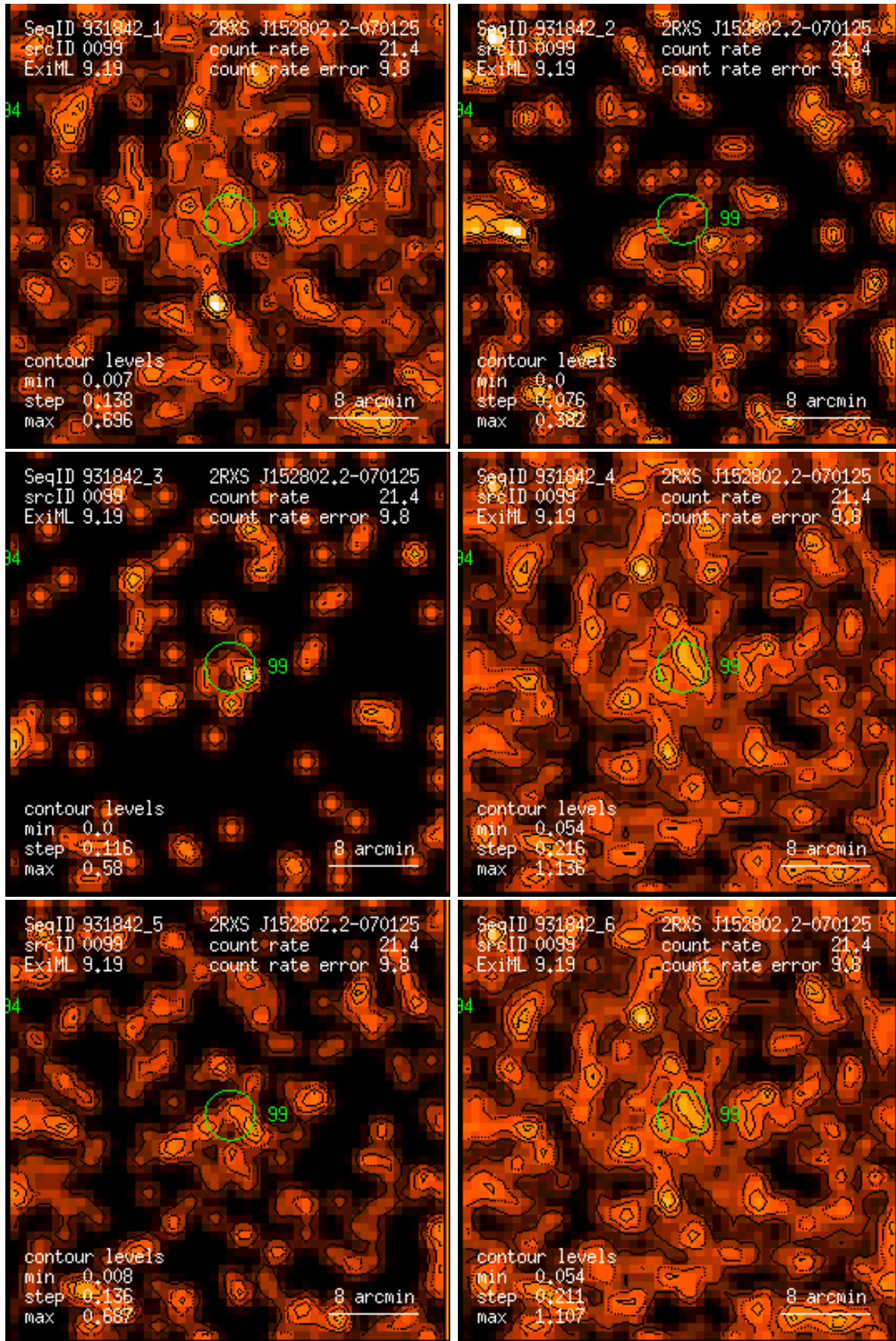
Figure 99: RASS 931842: detection 0099: band rate images, Gaussian filter: (1) PSPC channels 11 – 41, (2) 52 – 90, (3) 91 – 201, (4) 11 – 235, (5) 52 – 201, (6) 11 – 201. Broad band rates in counts/ks. Band rate contour levels in counts/ks/arcmin 2 .
