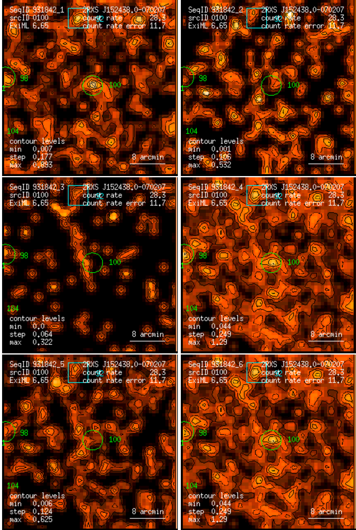
Figure 100: RASS 931842: detection 0100: band rate images, Gaussian filter: (1) PSPC channels 11 – 41, (2) 52 – 90, (3) 91 – 201, (4) 11 – 235, (5) 52 – 201, (6) 11 – 201. Broad band rates in counts/ks. Band rate contour levels in counts/ks/arcmin 2 .
