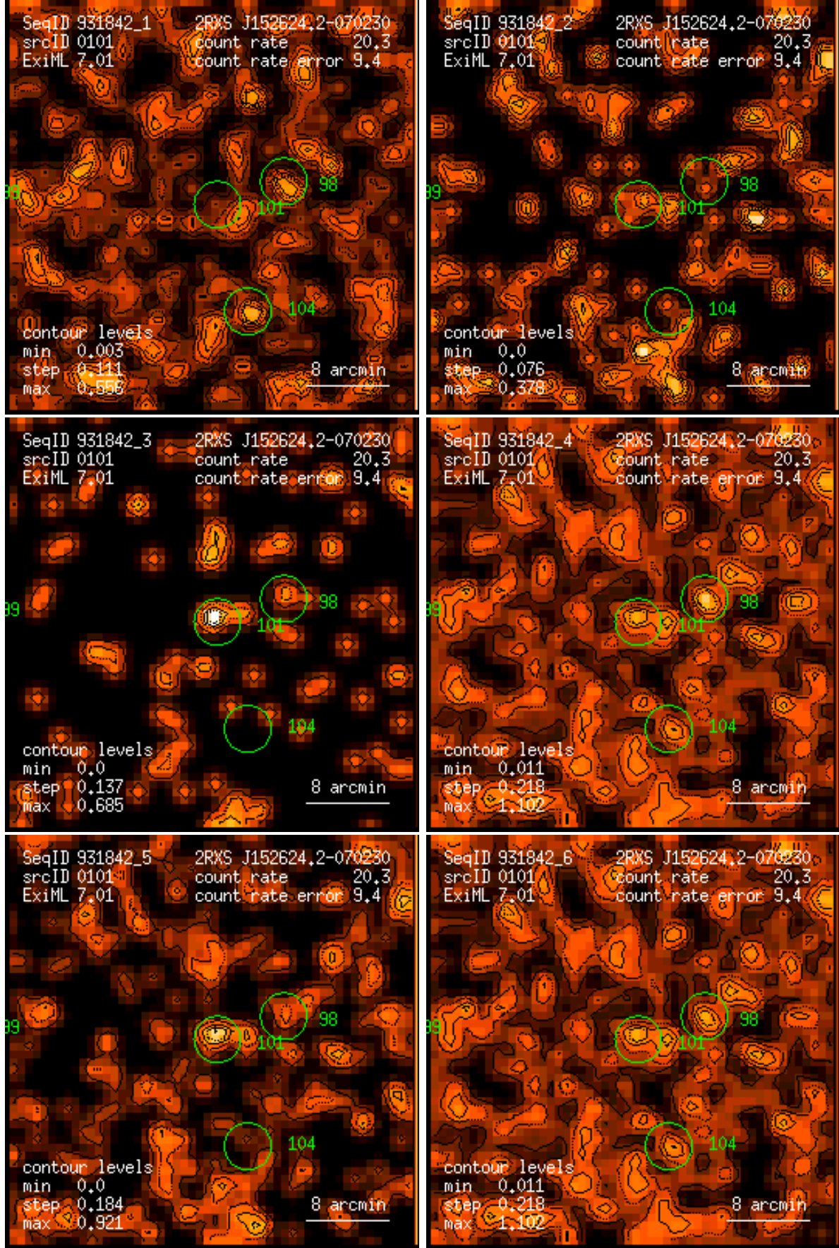
Figure 101: RASS 931842: detection 0101: band rate images, Gaussian filter: (1) PSPC channels 11 – 41, (2) 52 – 90, (3) 91 – 201, (4) 11 – 235, (5) 52 – 201, (6) 11 – 201. Broad band rates in counts/ks. Band rate contour levels in counts/ks/arcmin 2 .
