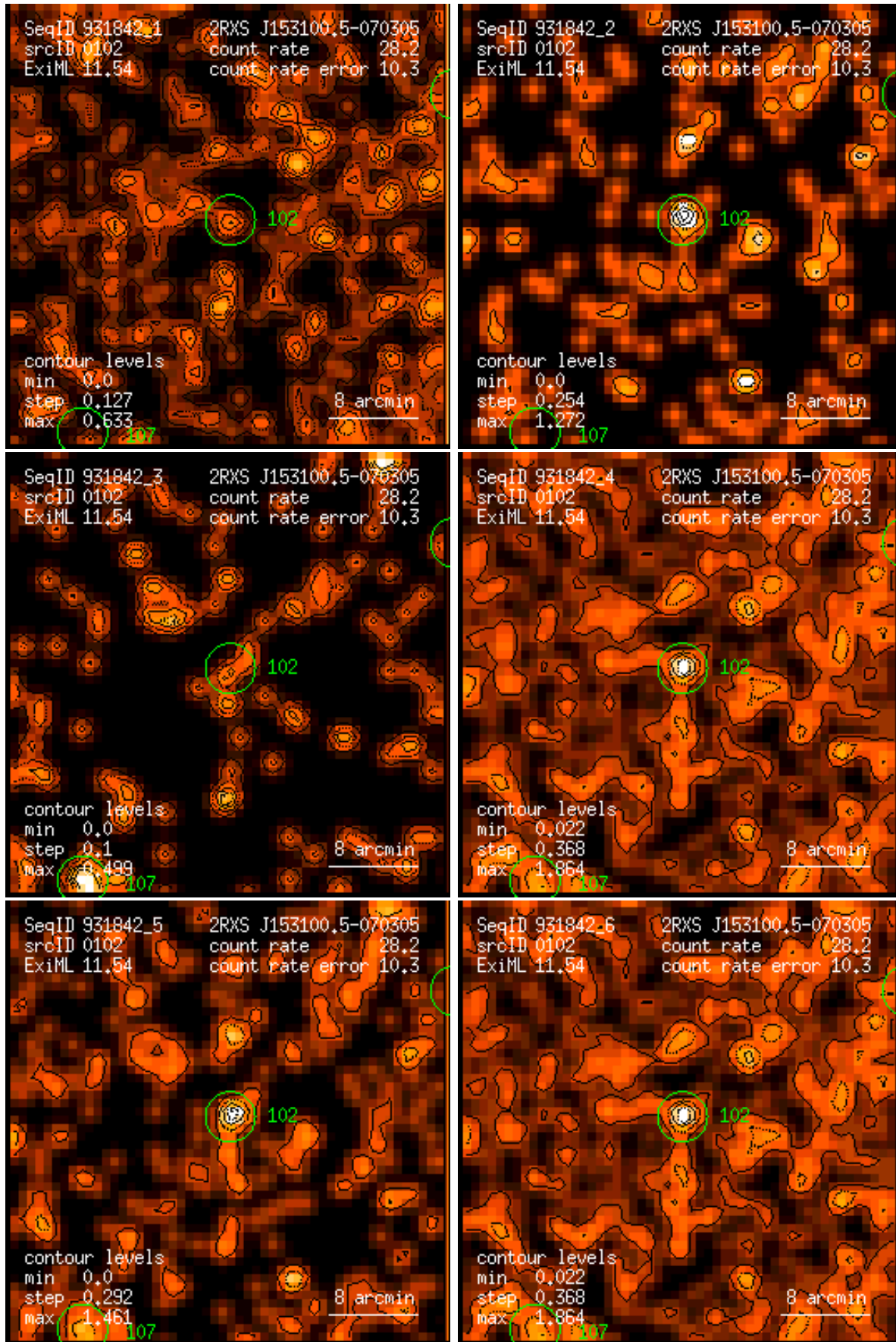
Figure 102: RASS 931842: detection 0102: band rate images, Gaussian filter: (1) PSPC channels 11 – 41, (2) 52 – 90, (3) 91 – 201, (4) 11 – 235, (5) 52 – 201, (6) 11 – 201. Broad band rates in counts/ks. Band rate contour levels in counts/ks/arcmin 2 .
