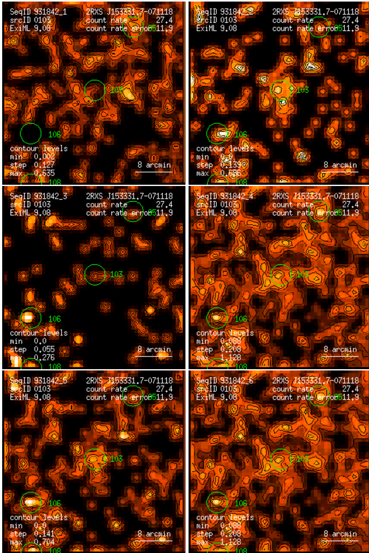
Figure 103: RASS 931842: detection 0103: band rate images, Gaussian filter: (1) PSPC channels 11 – 41, (2) 52 – 90, (3) 91 – 201, (4) 11 – 235, (5) 52 – 201, (6) 11 – 201. Broad band rates in counts/ks. Band rate contour levels in counts/ks/arcmin 2 .
