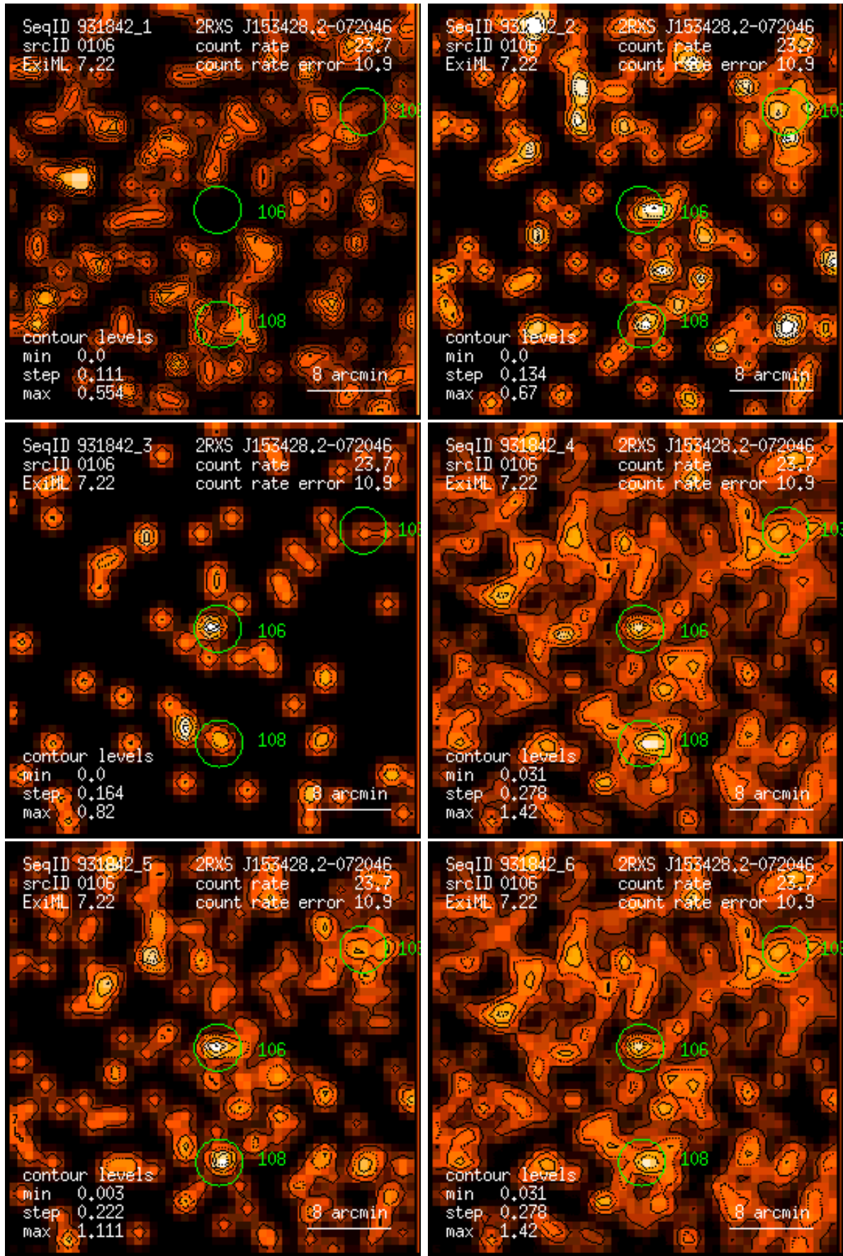
Figure 106: RASS 931842: detection 0106: band rate images, Gaussian filter: (1) PSPC channels 11 – 41, (2) 52 – 90, (3) 91 – 201, (4) 11 – 235, (5) 52 – 201, (6) 11 – 201. Broad band rates in counts/ks. Band rate contour levels in counts/ks/arcmin 2 .
