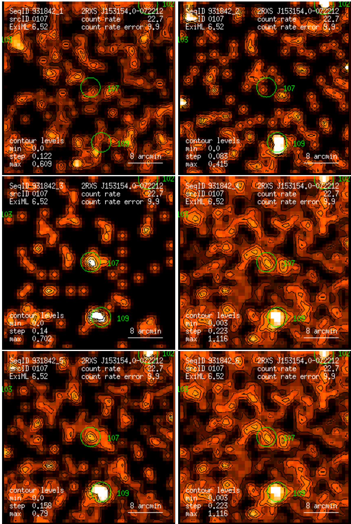
Figure 107: RASS 931842: detection 0107: band rate images, Gaussian filter: (1) PSPC channels 11 – 41, (2) 52 – 90, (3) 91 – 201, (4) 11 – 235, (5) 52 – 201, (6) 11 – 201. Broad band rates in counts/ks. Band rate contour levels in counts/ks/arcmin 2 .
