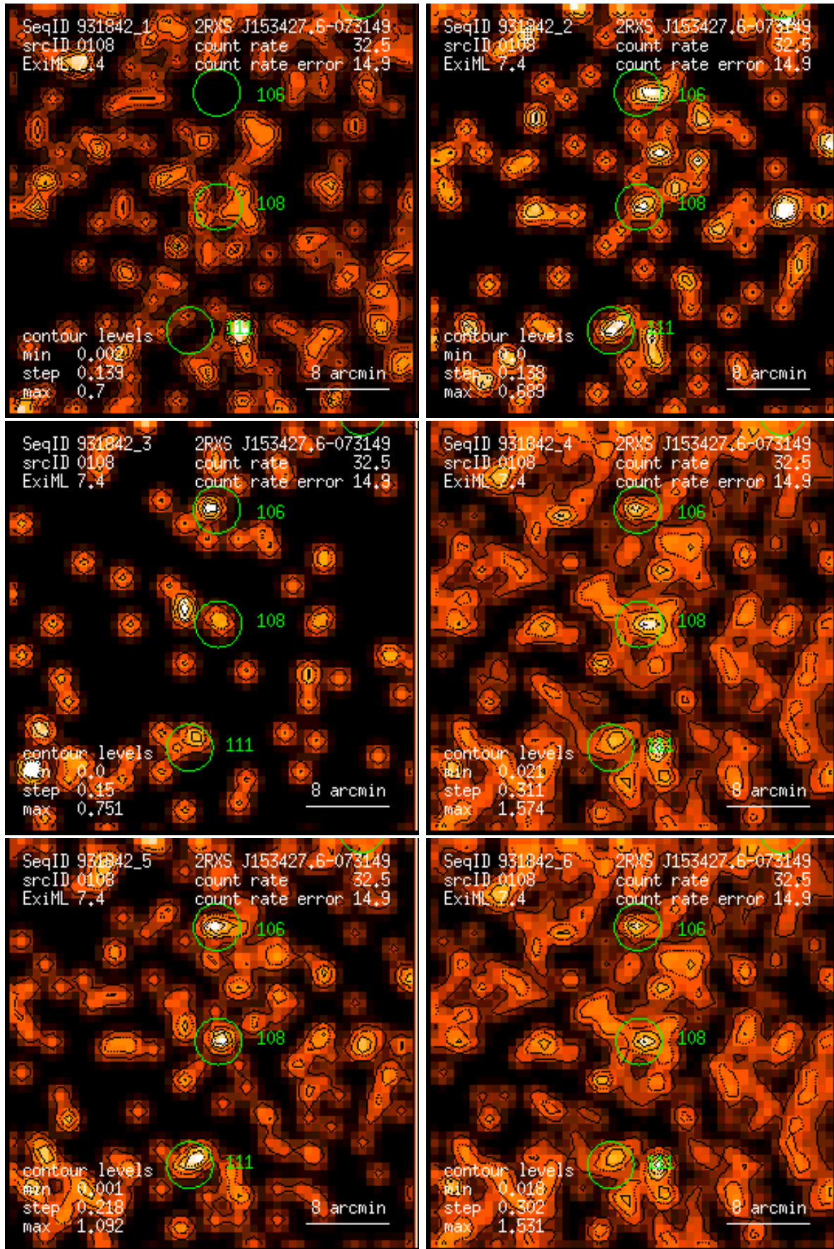
Figure 108: RASS 931842: detection 0108: band rate images, Gaussian filter: (1) PSPC channels 11 – 41, (2) 52 – 90, (3) 91 – 201, (4) 11 – 235, (5) 52 – 201, (6) 11 – 201. Broad band rates in counts/ks. Band rate contour levels in counts/ks/arcmin 2 .
