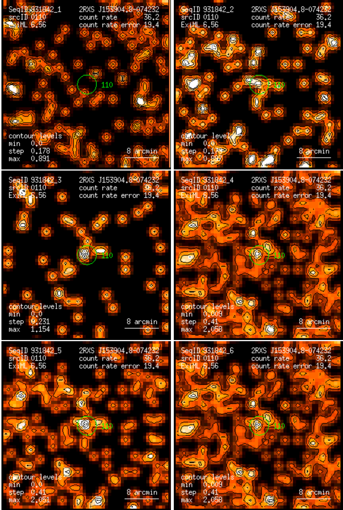
Figure 110: RASS 931842: detection 0110: band rate images, Gaussian filter: (1) PSPC channels 11 – 41, (2) 52 – 90, (3) 91 – 201, (4) 11 – 235, (5) 52 – 201, (6) 11 – 201. Broad band rates in counts/ks. Band rate contour levels in counts/ks/arcmin 2 .
