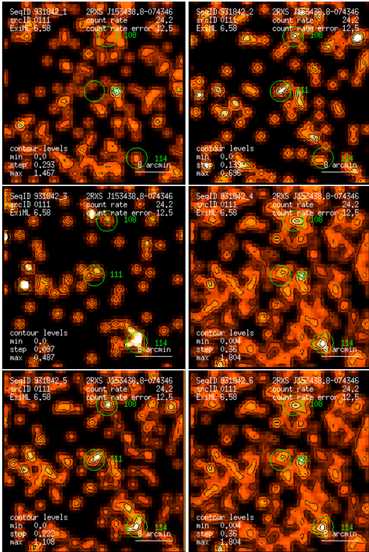
Figure 111: RASS 931842: detection 0111: band rate images, Gaussian filter: (1) PSPC channels 11 – 41, (2) 52 – 90, (3) 91 – 201, (4) 11 – 235, (5) 52 – 201, (6) 11 – 201. Broad band rates in counts/ks. Band rate contour levels in counts/ks/arcmin 2 .
