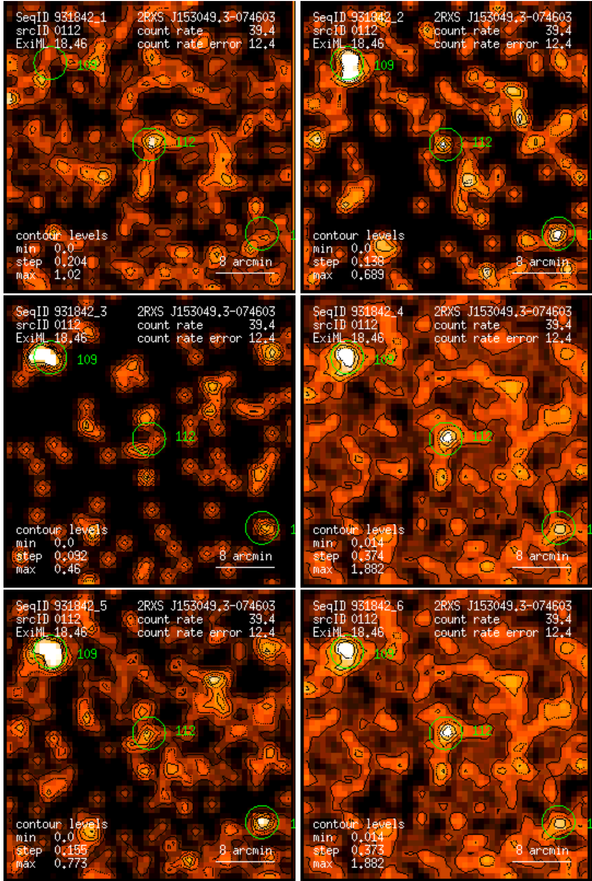
Figure 112: RASS 931842: detection 0112: band rate images, Gaussian filter: (1) PSPC channels 11 – 41, (2) 52 – 90, (3) 91 – 201, (4) 11 – 235, (5) 52 – 201, (6) 11 – 201. Broad band rates in counts/ks. Band rate contour levels in counts/ks/arcmin 2 .
