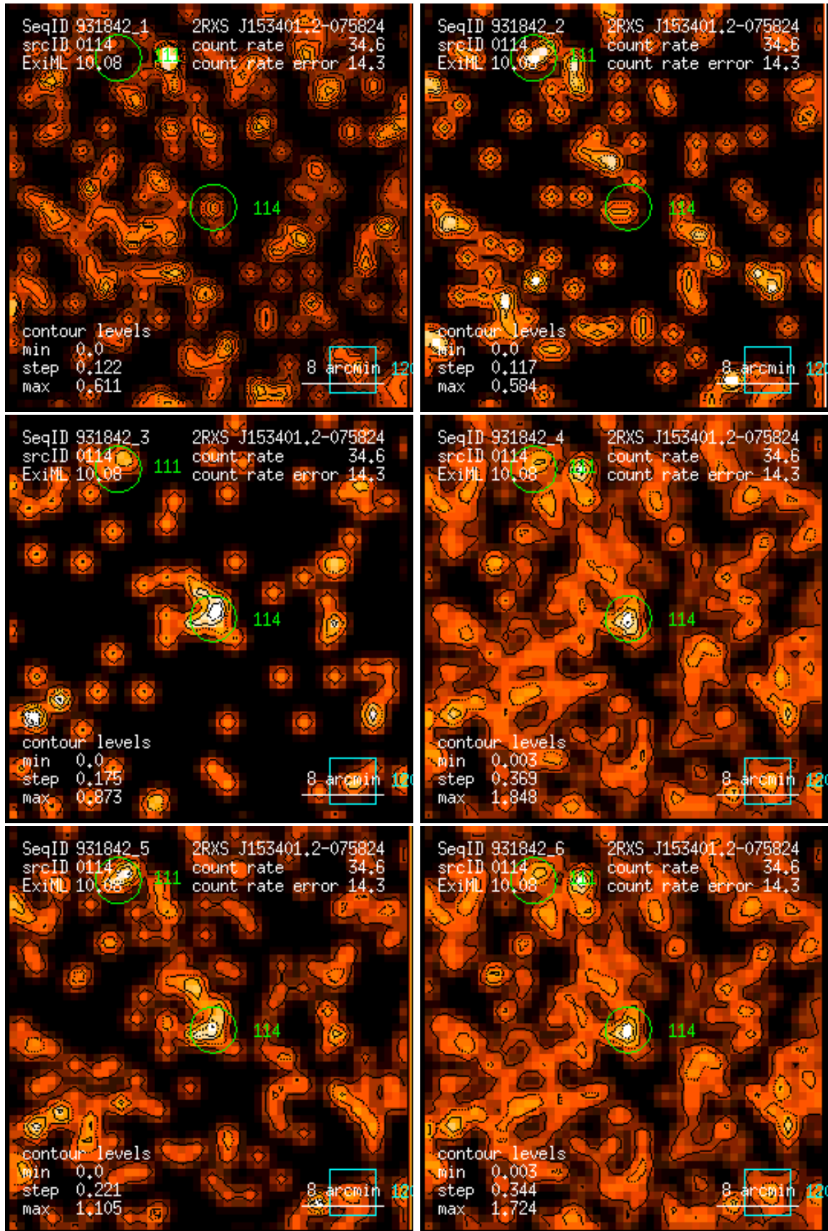
Figure 114: RASS 931842: detection 0114: band rate images, Gaussian filter: (1) PSPC channels 11 – 41, (2) 52 – 90, (3) 91 – 201, (4) 11 – 235, (5) 52 – 201, (6) 11 – 201. Broad band rates in counts/ks. Band rate contour levels in counts/ks/arcmin 2 .
