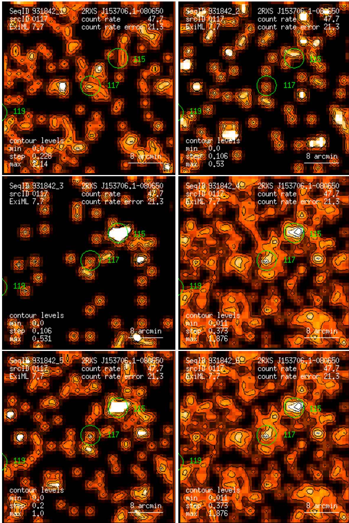
Figure 117: RASS 931842: detection 0117: band rate images, Gaussian filter: (1) PSPC channels 11 – 41, (2) 52 – 90, (3) 91 – 201, (4) 11 – 235, (5) 52 – 201, (6) 11 – 201. Broad band rates in counts/ks. Band rate contour levels in counts/ks/arcmin 2 .
