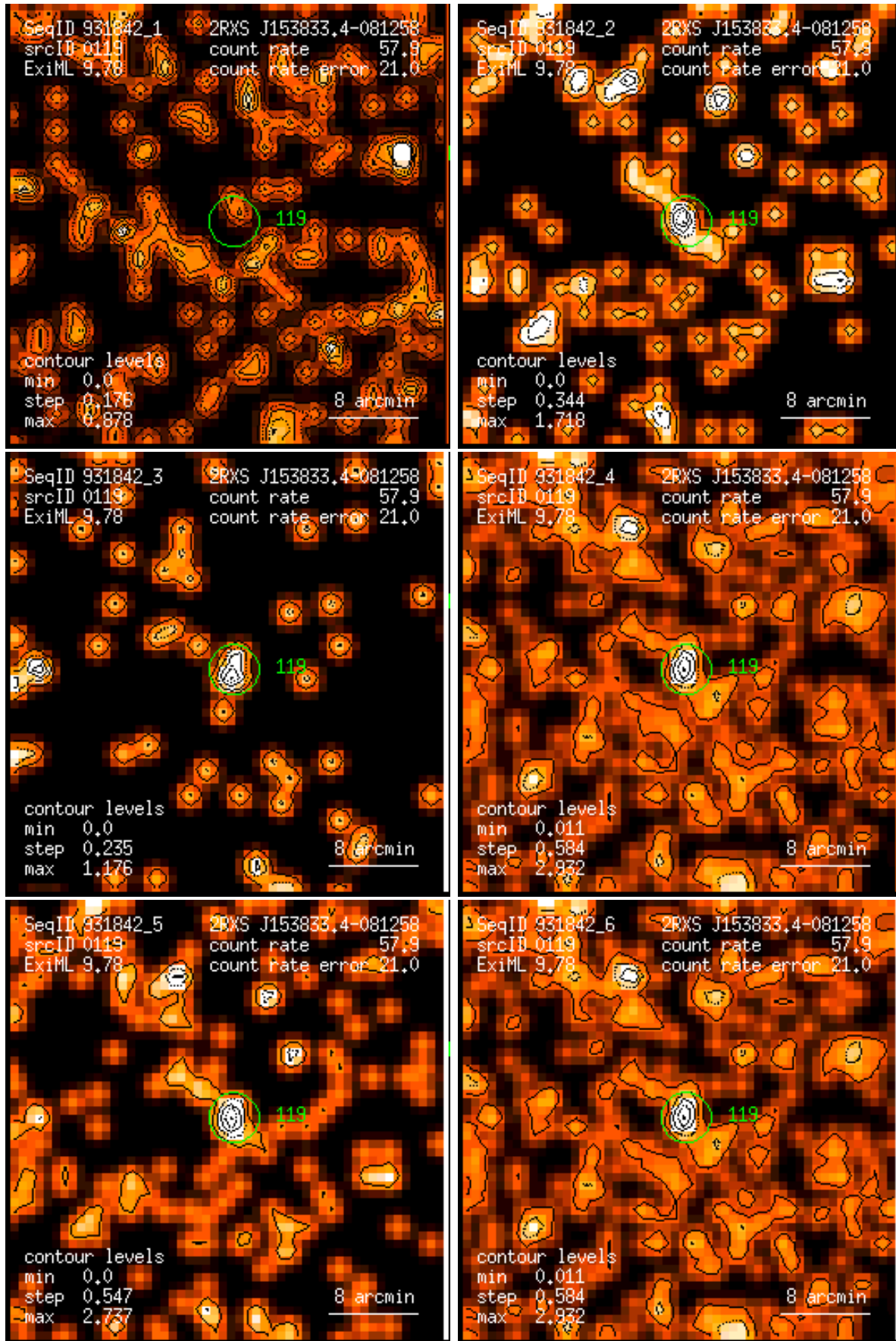
Figure 119: RASS 931842: detection 0119: band rate images, Gaussian filter: (1) PSPC channels 11 – 41, (2) 52 – 90, (3) 91 – 201, (4) 11 – 235, (5) 52 – 201, (6) 11 – 201. Broad band rates in counts/ks. Band rate contour levels in counts/ks/arcmin 2 .
