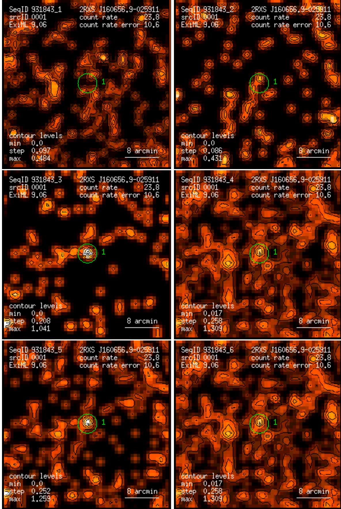
Figure 1: RASS 931843: detection 0001: band rate images, Gaussian filter: (1) PSPC channels 11 – 41, (2) 52 – 90, (3) 91 – 201, (4) 11 – 235, (5) 52 – 201, (6) 11 – 201. Broad band rates in counts/ks. Band rate contour levels in counts/ks/arcmin 2 .
