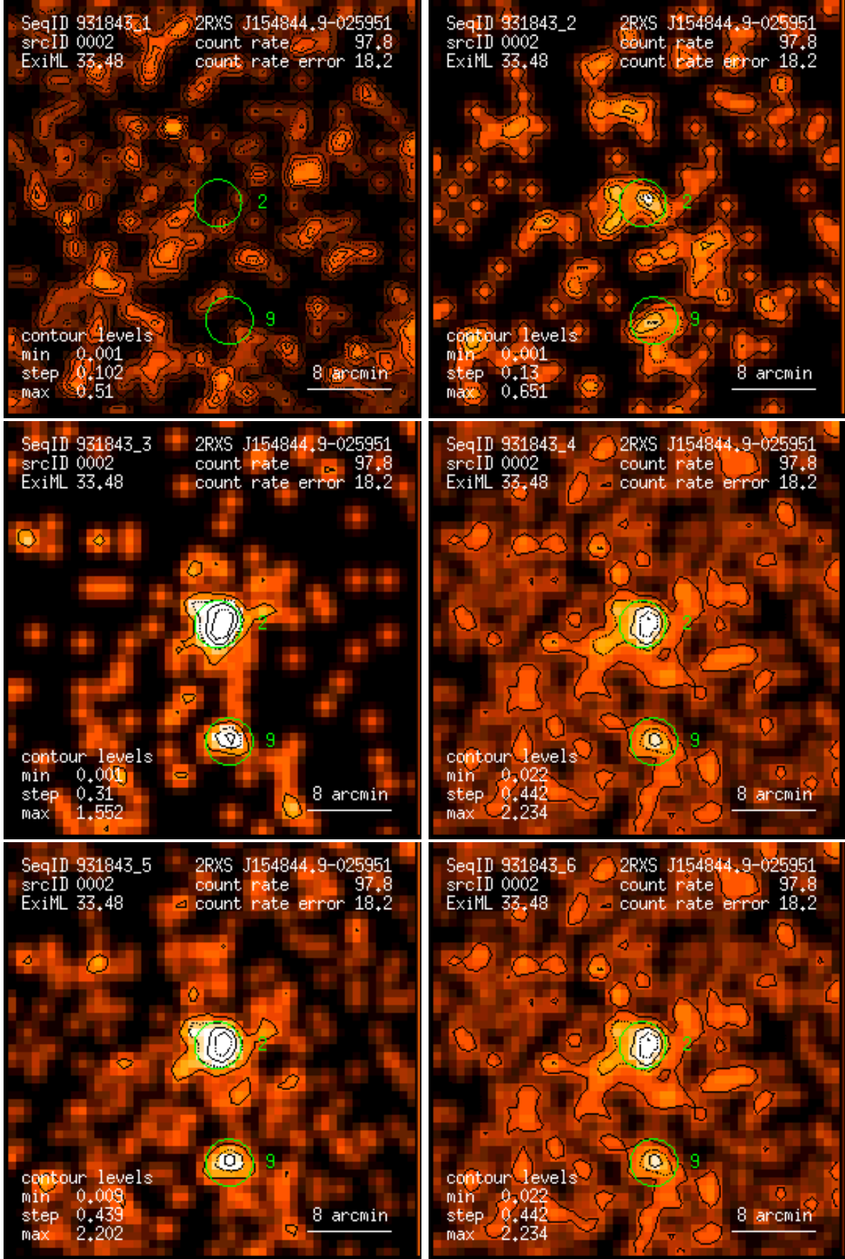
Figure 2: RASS 931843: detection 0002: band rate images, Gaussian filter: (1) PSPC channels 11 – 41, (2) 52 – 90, (3) 91 – 201, (4) 11 – 235, (5) 52 – 201, (6) 11 – 201. Broad band rates in counts/ks. Band rate contour levels in counts/ks/arcmin 2 .
