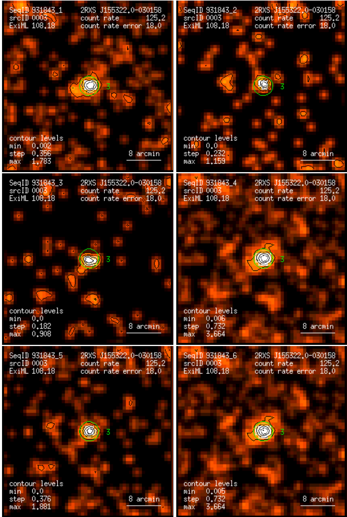
Figure 3: RASS 931843: detection 0003: band rate images, Gaussian filter: (1) PSPC channels 11 – 41, (2) 52 – 90, (3) 91 – 201, (4) 11 – 235, (5) 52 – 201, (6) 11 – 201. Broad band rates in counts/ks. Band rate contour levels in counts/ks/arcmin 2 .
