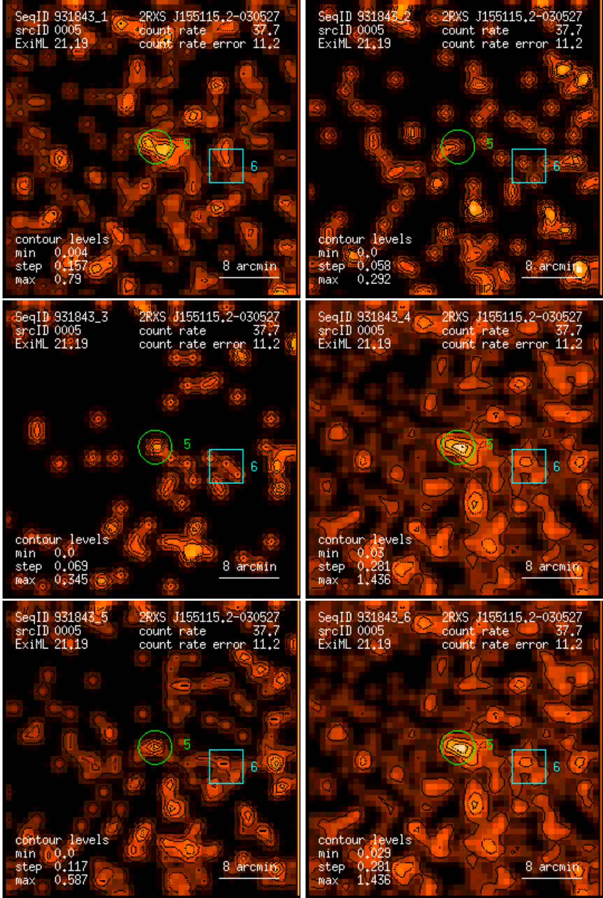
Figure 5: RASS 931843: detection 0005: band rate images, Gaussian filter: (1) PSPC channels 11 – 41, (2) 52 – 90, (3) 91 – 201, (4) 11 – 235, (5) 52 – 201, (6) 11 – 201. Broad band rates in counts/ks. Band rate contour levels in counts/ks/arcmin 2 .
