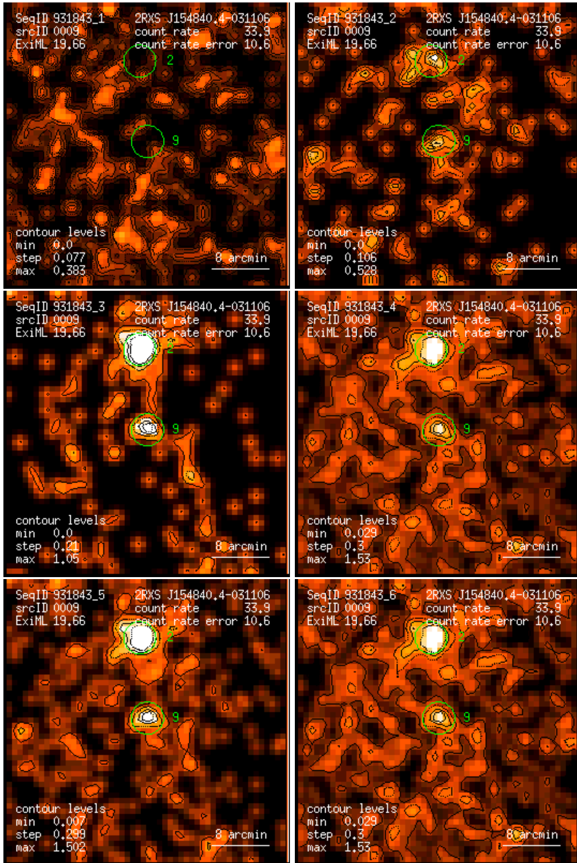
Figure 9: RASS 931843: detection 0009: band rate images, Gaussian filter: (1) PSPC channels 11 – 41, (2) 52 – 90, (3) 91 – 201, (4) 11 – 235, (5) 52 – 201, (6) 11 – 201. Broad band rates in counts/ks. Band rate contour levels in counts/ks/arcmin 2 .
