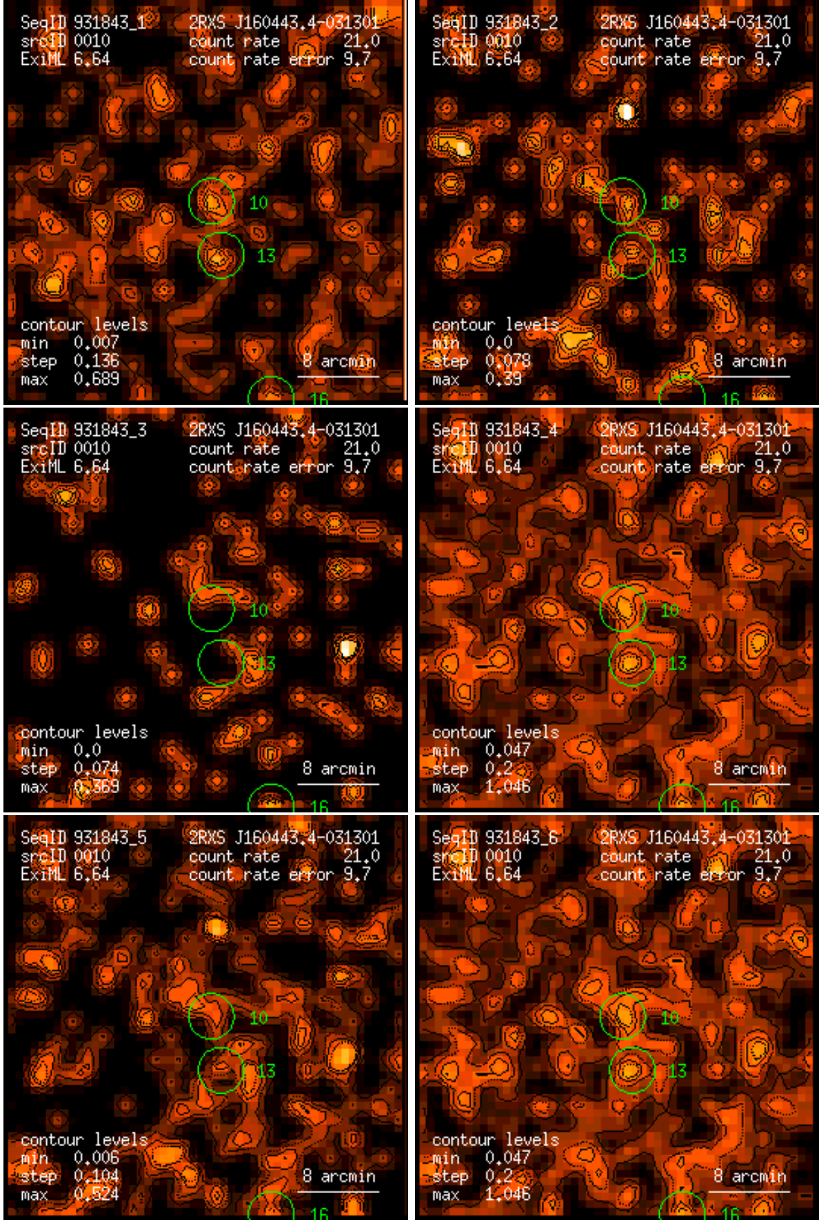
Figure 10: RASS 931843: detection 0010: band rate images, Gaussian filter: (1) PSPC channels 11 – 41, (2) 52 – 90, (3) 91 – 201, (4) 11 – 235, (5) 52 – 201, (6) 11 – 201. Broad band rates in counts/ks. Band rate contour levels in counts/ks/arcmin 2 .
