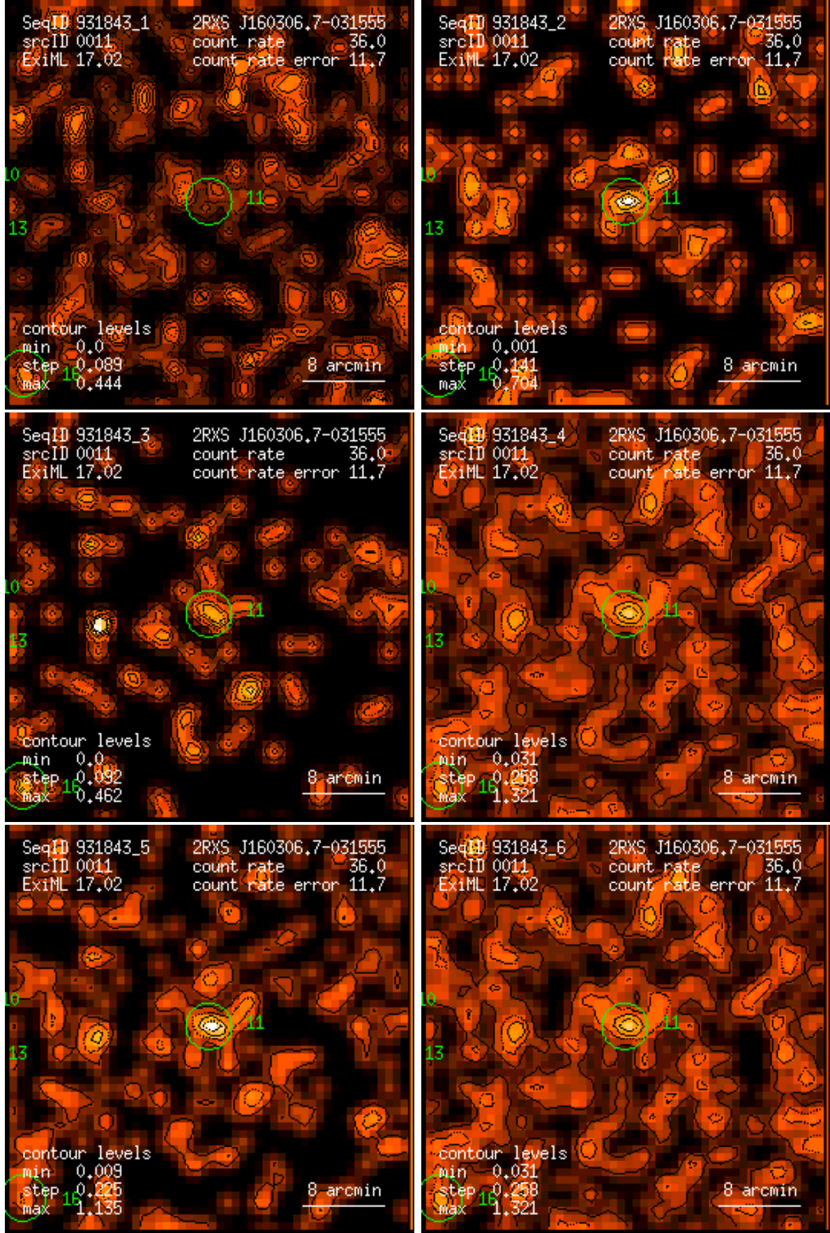
Figure 11: RASS 931843: detection 0011: band rate images, Gaussian filter: (1) PSPC channels 11 – 41, (2) 52 – 90, (3) 91 – 201, (4) 11 – 235, (5) 52 – 201, (6) 11 – 201. Broad band rates in counts/ks. Band rate contour levels in counts/ks/arcmin 2 .
