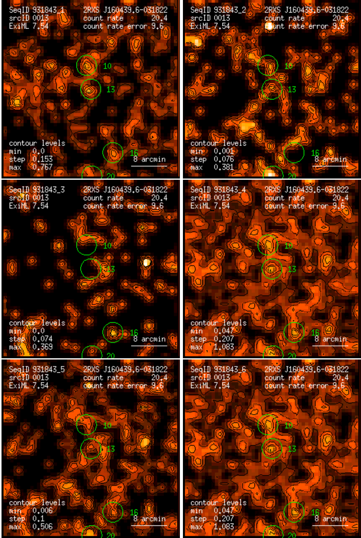
Figure 13: RASS 931843: detection 0013: band rate images, Gaussian filter: (1) PSPC channels 11 – 41, (2) 52 – 90, (3) 91 – 201, (4) 11 – 235, (5) 52 – 201, (6) 11 – 201. Broad band rates in counts/ks. Band rate contour levels in counts/ks/arcmin 2 .
