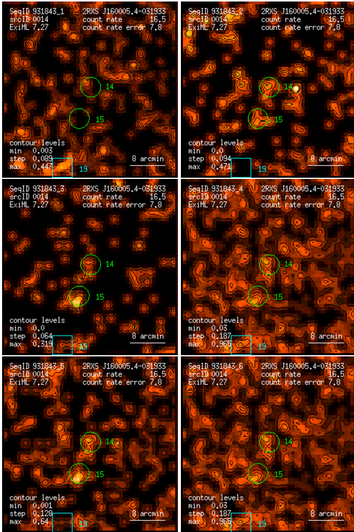
Figure 14: RASS 931843: detection 0014: band rate images, Gaussian filter: (1) PSPC channels 11 – 41, (2) 52 – 90, (3) 91 – 201, (4) 11 – 235, (5) 52 – 201, (6) 11 – 201. Broad band rates in counts/ks. Band rate contour levels in counts/ks/arcmin 2 .
