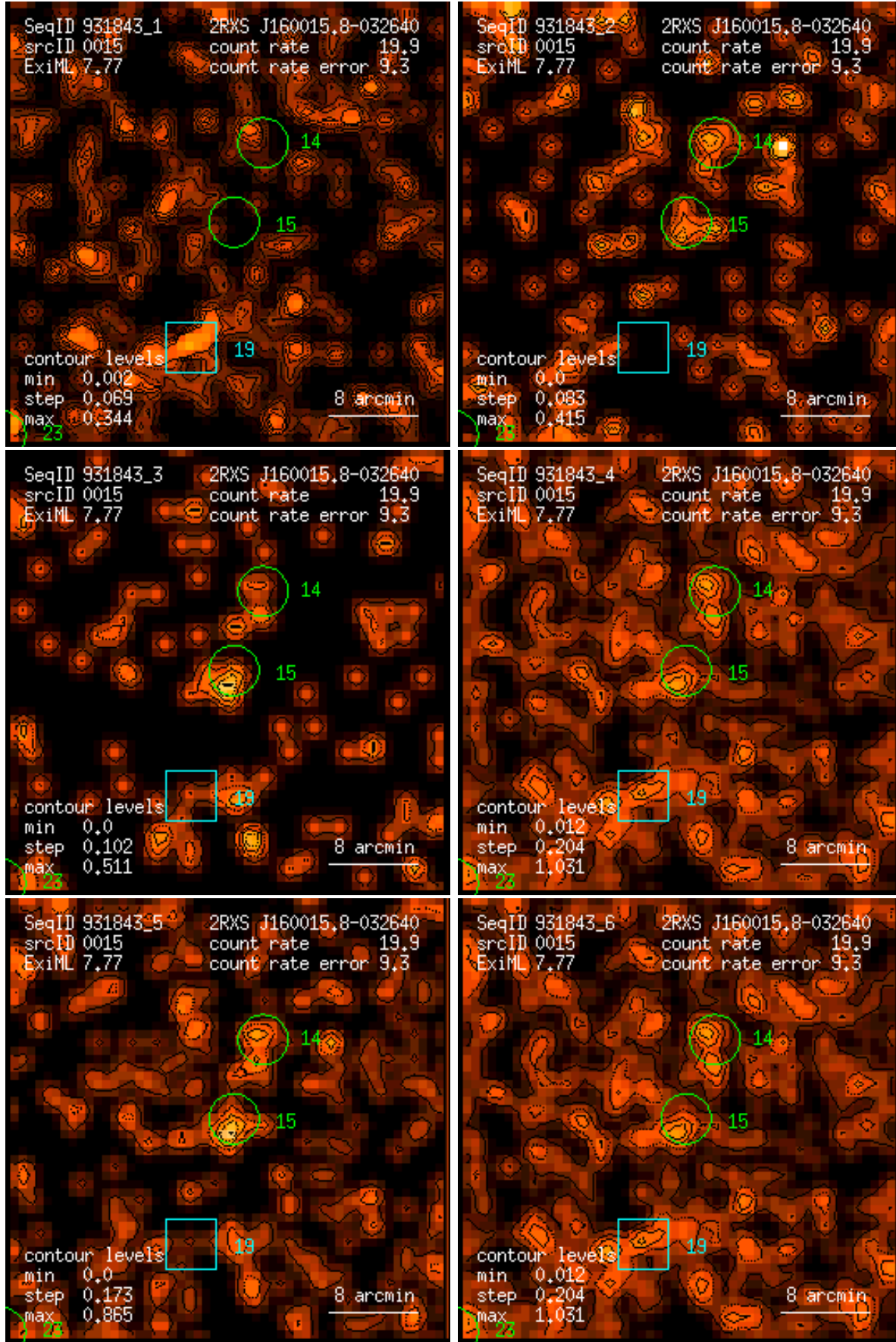
Figure 15: RASS 931843: detection 0015: band rate images, Gaussian filter: (1) PSPC channels 11 – 41, (2) 52 – 90, (3) 91 – 201, (4) 11 – 235, (5) 52 – 201, (6) 11 – 201. Broad band rates in counts/ks. Band rate contour levels in counts/ks/arcmin 2 .
